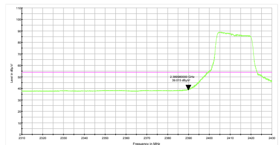
802.11g-Channel 1 Average
