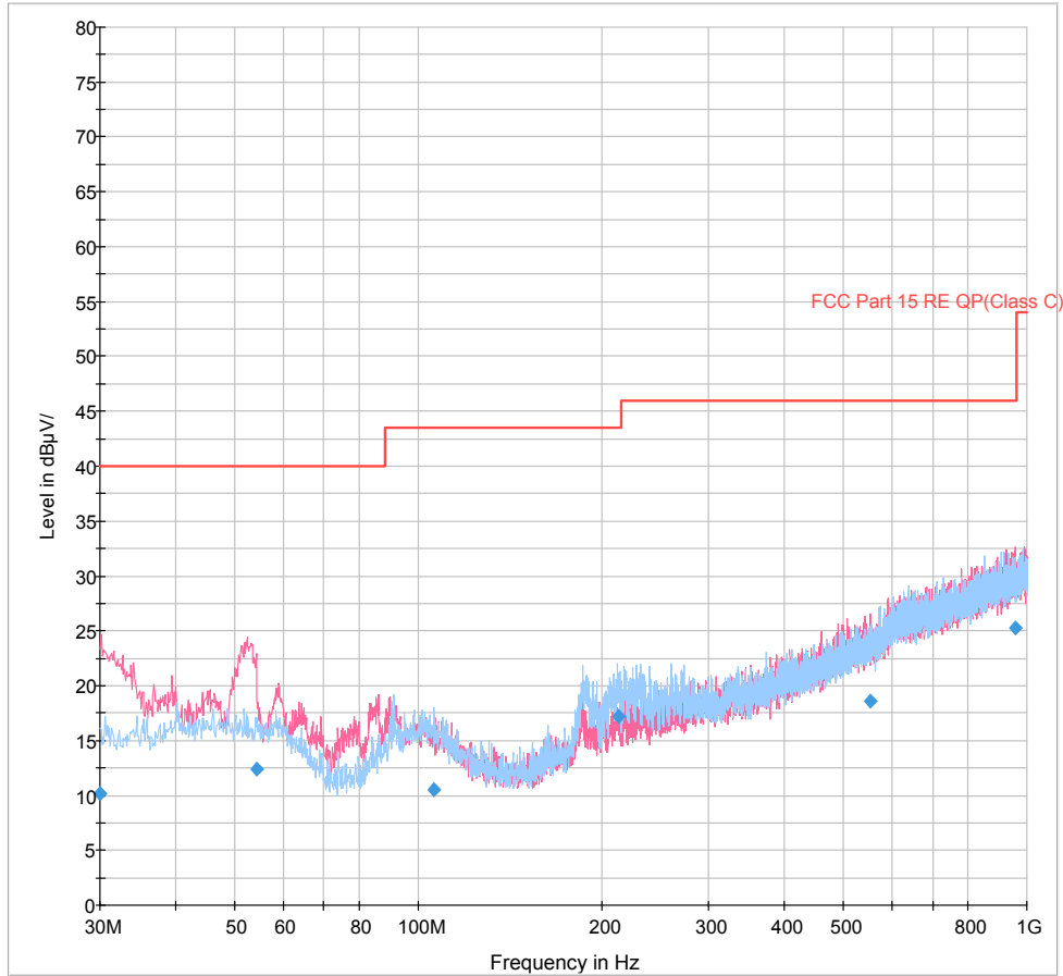
Radiates Emission from 30MHz to 1GHz
