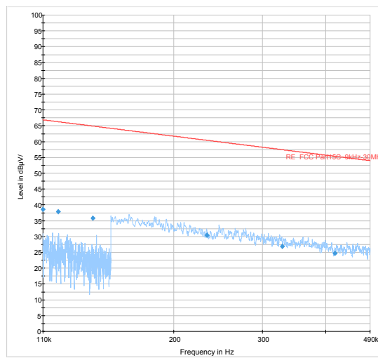
Radiates Emission from 110kHz to 490kHz
