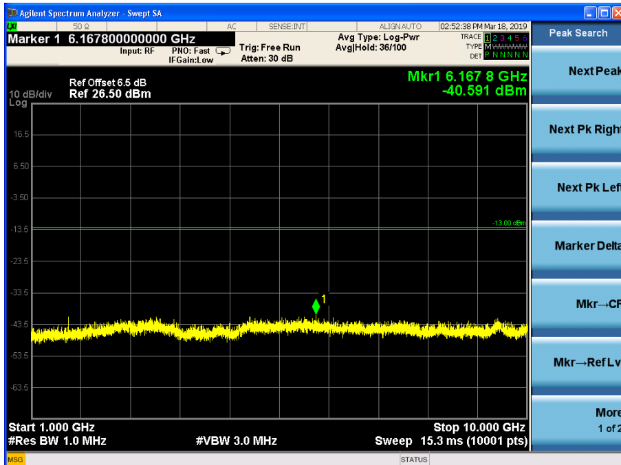
Channel 4183, 1GHz~10GHz
