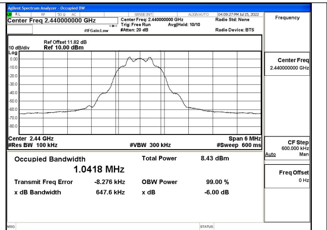
Test Mode:Coded 500K
