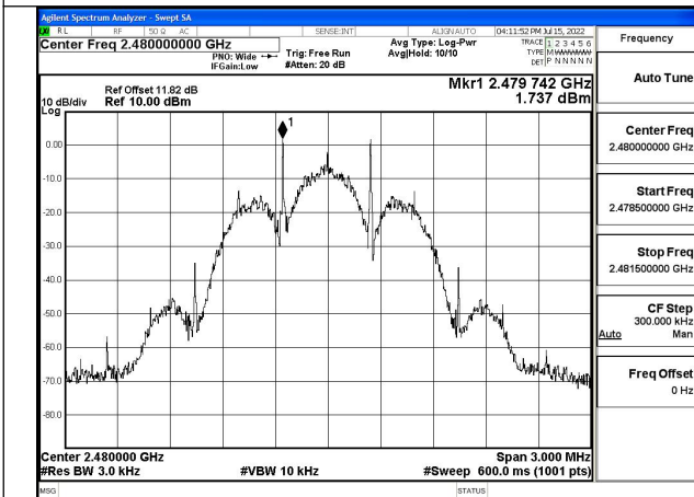
Test Mode:Coded 500K
