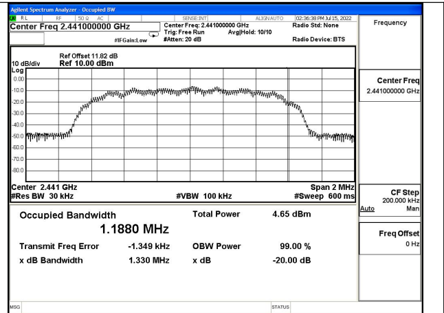
Test Mode: \pi /4DQPSK(2DH5)
