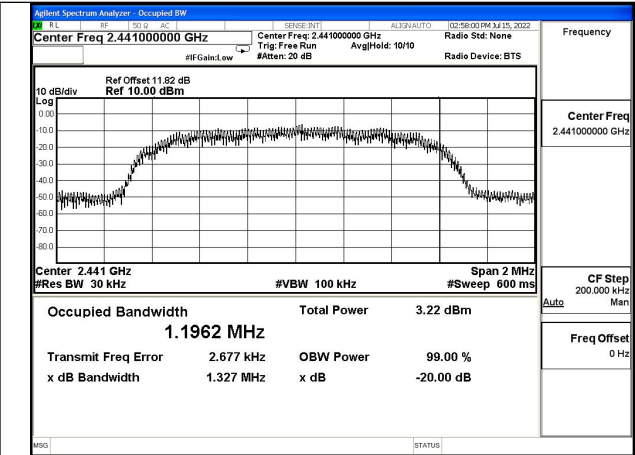
Test Mode:8DPSK(3DH5)
