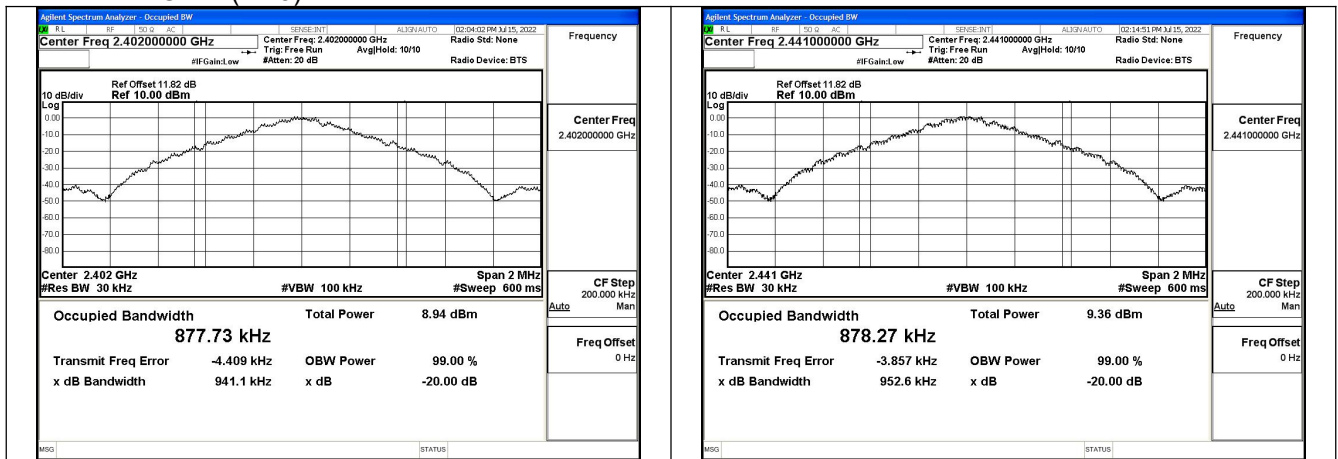
Test Mode:GFSK(DH5)
