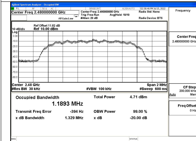
Test Mode: \pi /4DQPSK(2DH5)
