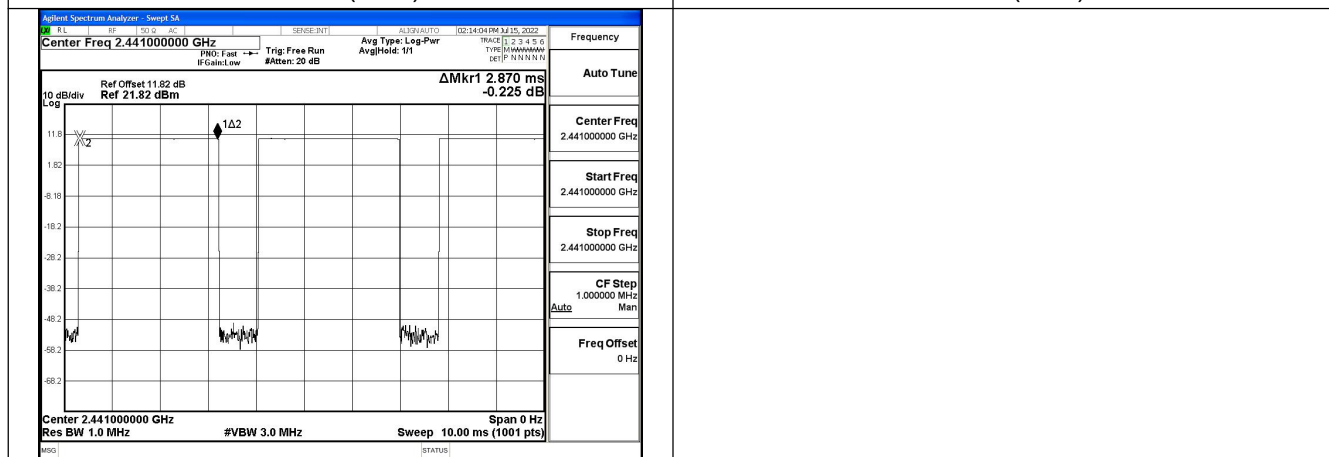
Test Mode:GFSK(DH5) 2441MHz
