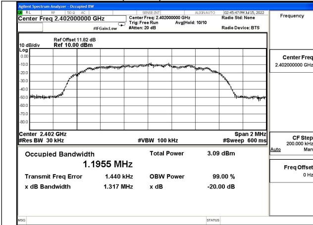
Test Mode:8DPSK(3DH5)
