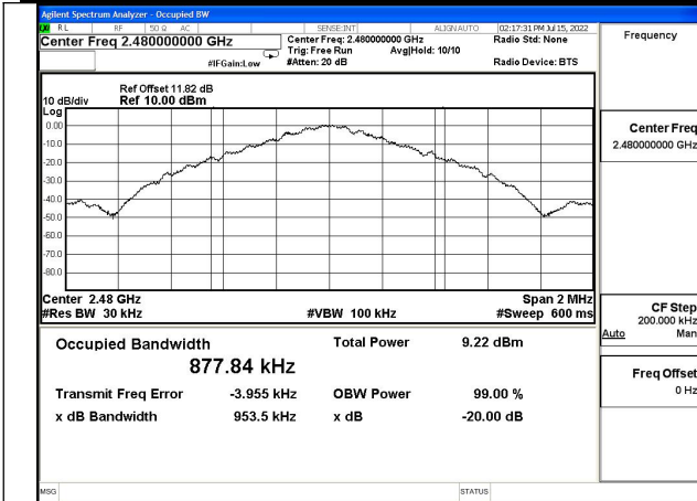
Test Mode:GFSK(DH5)
