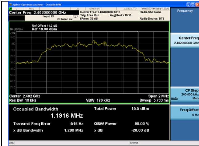
Modulation type: \pi/4 DQPSK2402MHz
