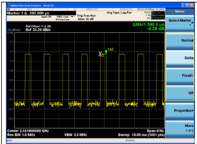
Modulation type: GFSK DH1 2441MHz
