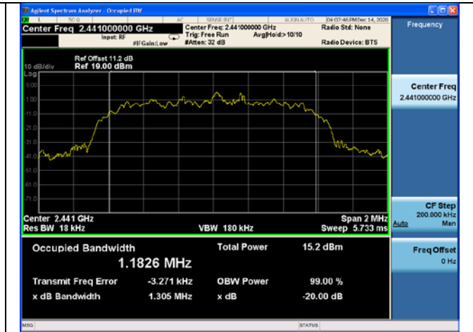
Modulation type: \pi/4 DQPSK2441MHz
