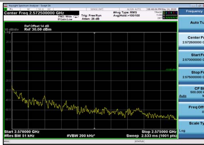
FDD07_10MHz_2565_Q16_OneRB_high_ExtraBands_Range_2570~2575
