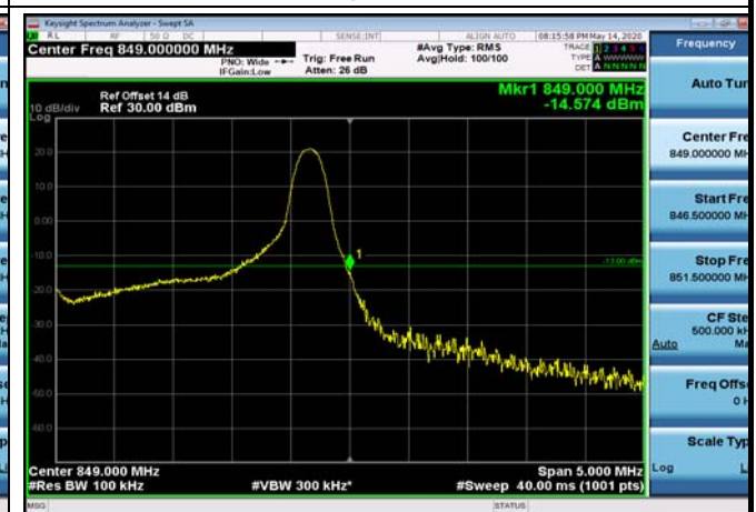
HighRange_FDD05_5MHz_846.5_fullRB_High_Q16
