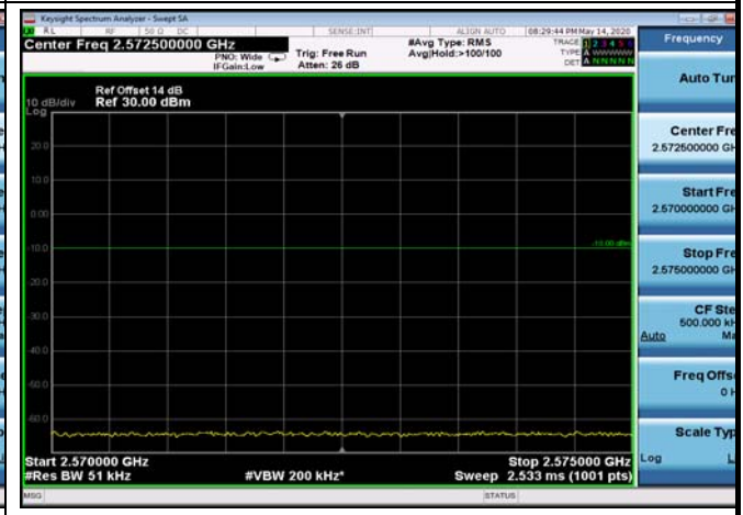
FDD07_10MHz_2505_Q16_fullIRB_ExtraBand_s_Range_2570~2575
