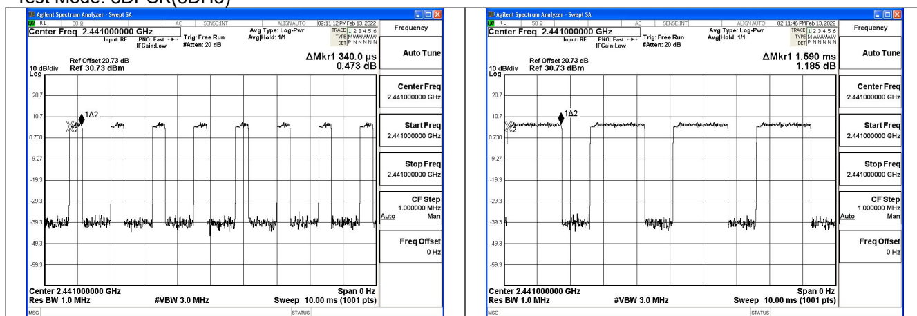
Test Mode:8DPSK(3DH1) 2441MHz
