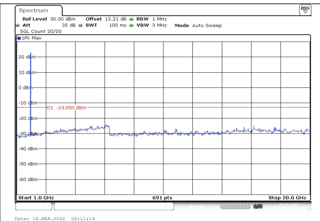
Channel 9262 1GHz~20GHz(dBm)
