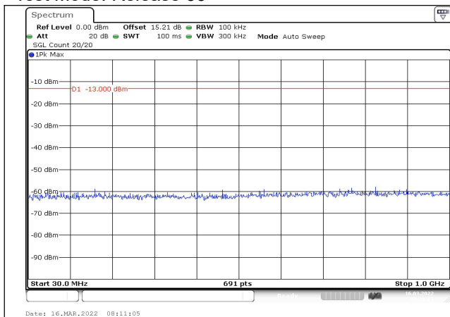
Channel 9262 30MHz~1GHz(dBm)
