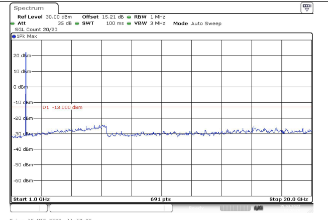
Channel 9262 1GHz~20GHz(dBm)
