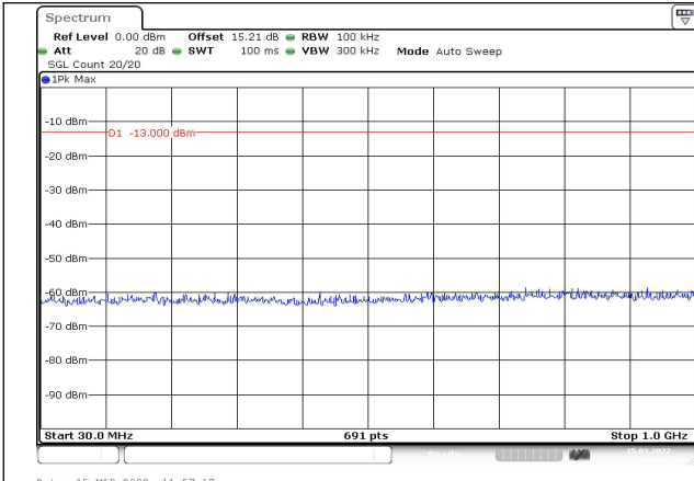
Channel 9262 30MHz~1GHz(dBm)
