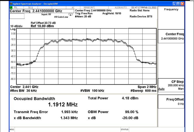
Test Mode:π/4DQPSK(2DH5) MHz
