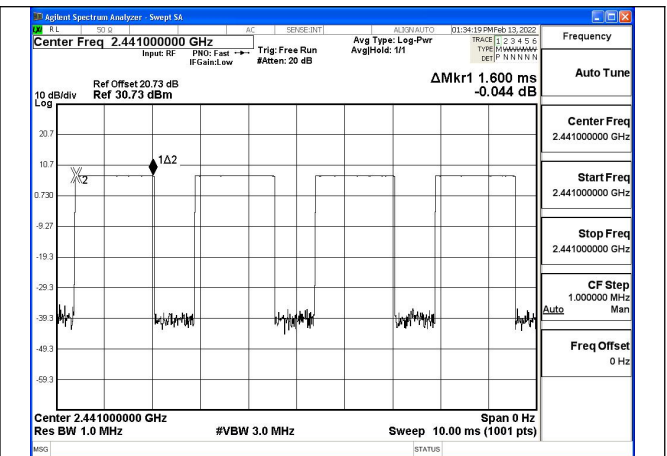
Test Mode:GFSK(DH3) 2441MHz
