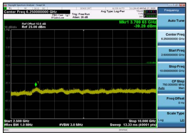
Conducted Emission: GFSK,2480,DH5 ,2500MHz~10000MHz
