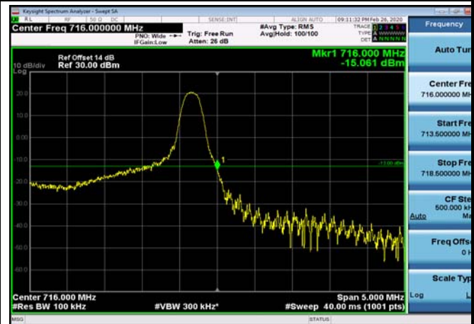
HighRange_FDD17_5MHz_713.5_OneRB _high_Q16
