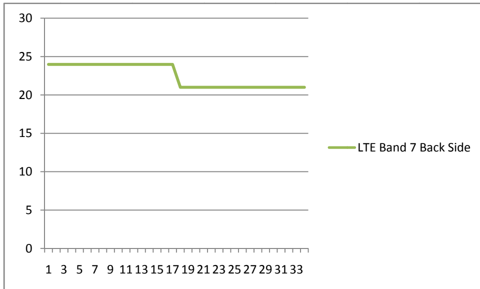
The DUT (Back side) is moved toward to the Phantom: Distance VS Output Power
