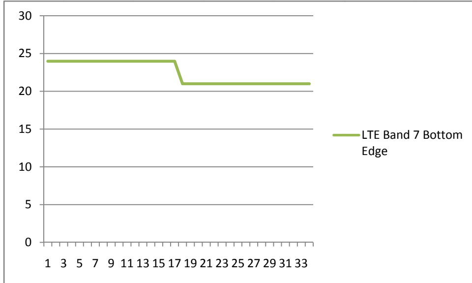
The DUT (bottom side) is moved toward to the Phantom: Distance VS Output Power
