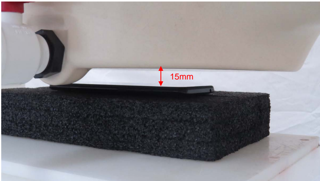
Picture 9: Front Side, the distance from handset to the bottom of the Phantom is 15mm
