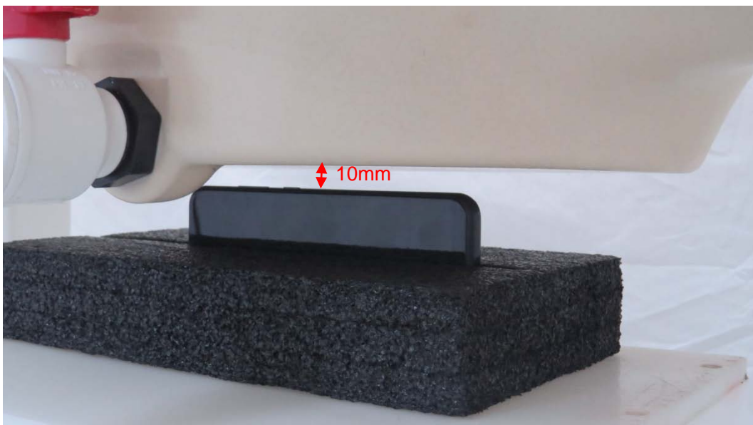
Picture 14: Right Side, the distance from handset to the bottom of the Phantom is 10mm
