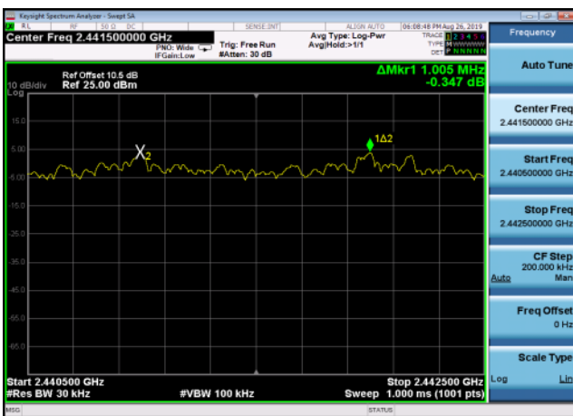
DQPSK,Hopping2DH5,2440.5~2442.5
