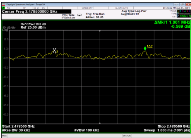
8DPSK,Hopping3DH5,2478.5~2480.5
