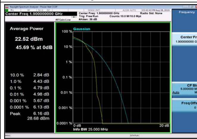
FDD02_HighRange_20MHz_1900_OneRB _high_Q16
