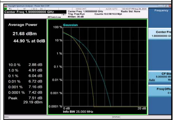
FDD02_HighRange_20MHz_1900_fullRB _Q16
