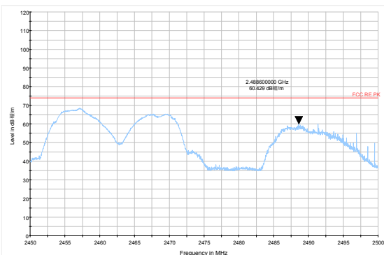
802.11g-Channel 11 Peak
