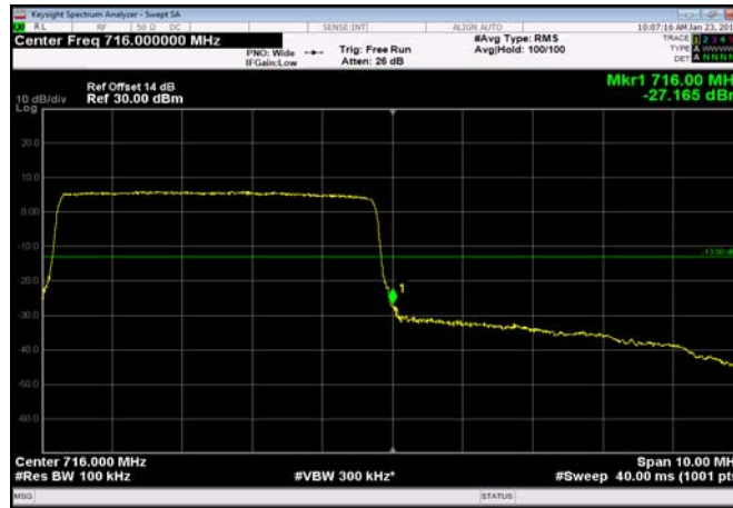
HighRange_FDD17_10MHz_711_OneRB _high_Q16
