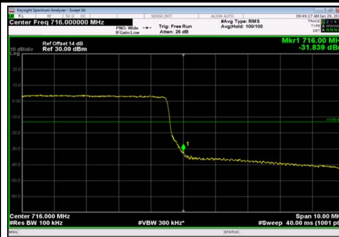
HighRange_FDD17_10MHz_711_fullRB _High_QPSK
