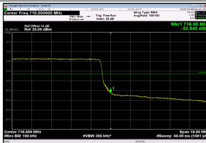
HighRange_FDD17_10MHz_711_fullRB _High_Q16
