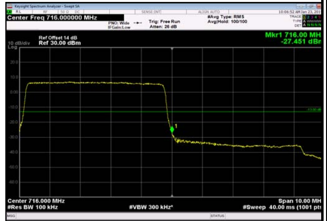
HighRange_FDD17_10MHz_711_OneRB _high_QPSK
