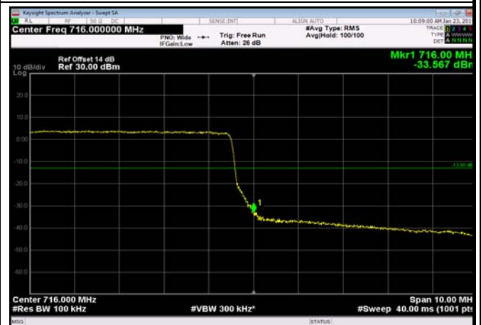
HighRange_FDD17_10MHz_711_fullRB _High_QPSK
