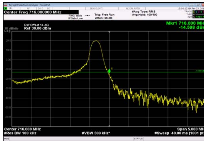
HighRange_FDD17_5MHz_713.5_OneRB _high_Q16
