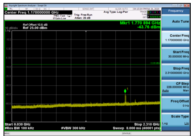
Conducted Emission: DQPSK,2402,2DH5 ,30MHz~2310MHz
