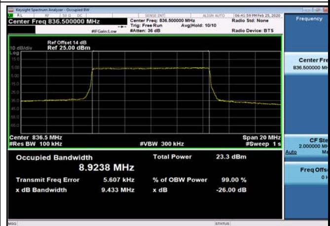
FDD05_MidRange_10MHz_836.5MHz_Q16
