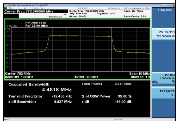
FDD13_MidRange_5_782_Q16
