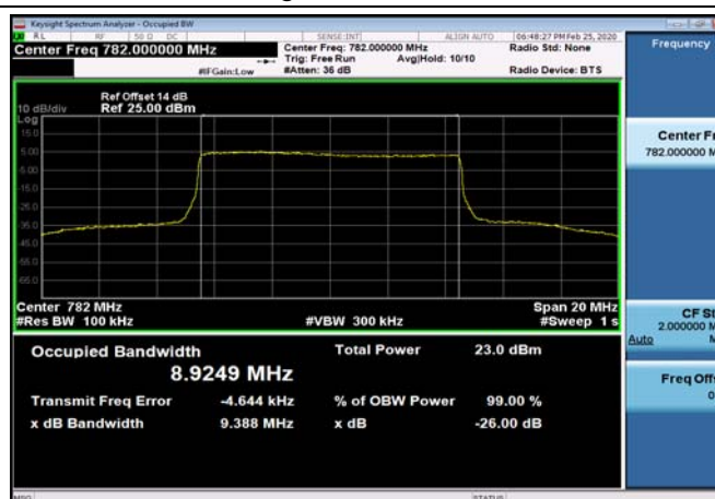
FDD13_MidRange_10MHz_782MHz_QPSK
