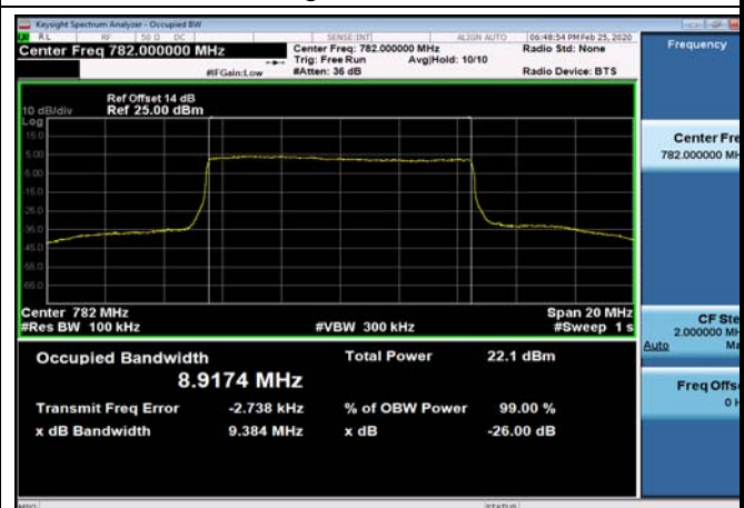
FDD13_MidRange_10MHz_782MHz_Q16
