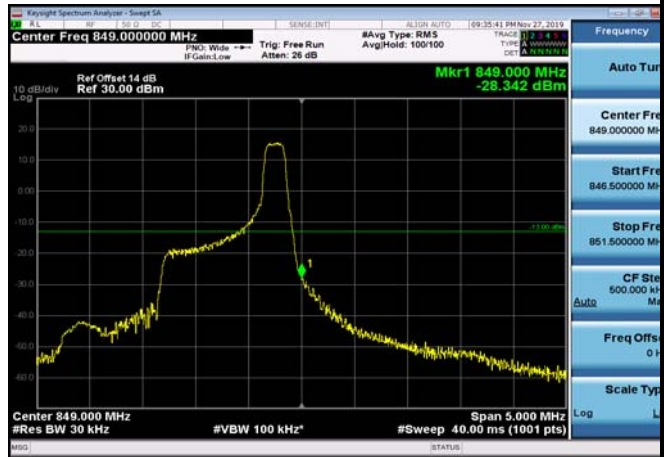
HighRange_FDD05_1.4MHz_848.3_fullRB_High_Q16
