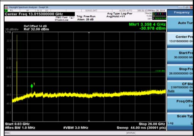
FDD05_HighRange_5MHz_30MHz~26GHz
