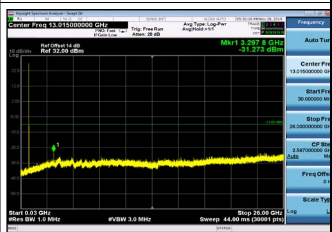
FDD05_LowRange_10MHz_30MHz~26GHz
