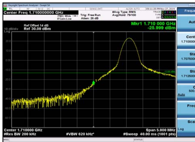
LowRange_FDD04_20MHz_1720_OneRB_low_QPSK
