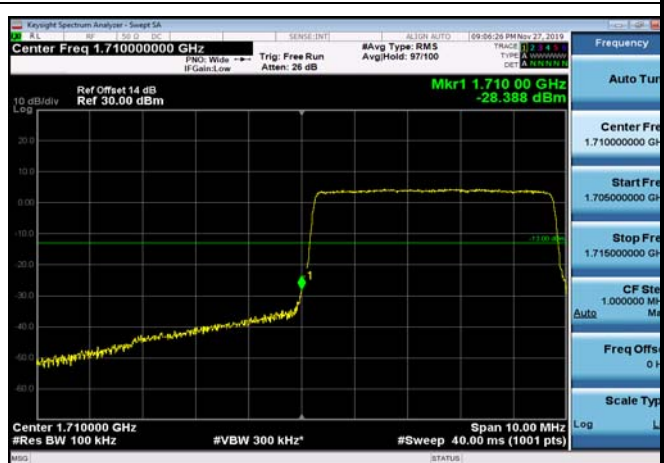
LowRange_FDD04_10MHz_1715_OneRB _low_Q16
