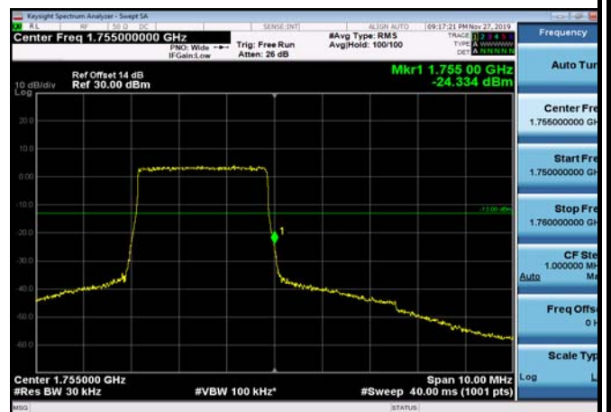
HighRange_FDD04_5MHz_1752.5_OneRB_high_Q16
