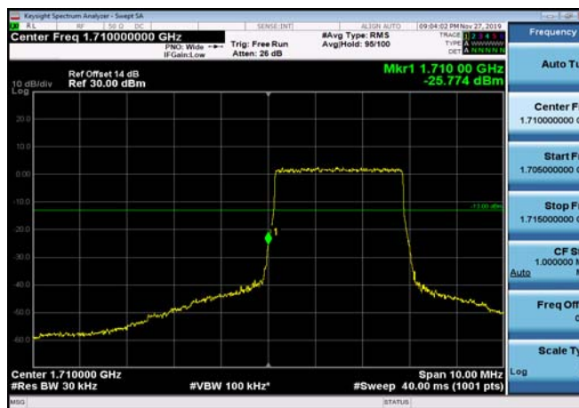
LowRange_FDD04_5MHz_1712.5_OneRB_low_QPSK
