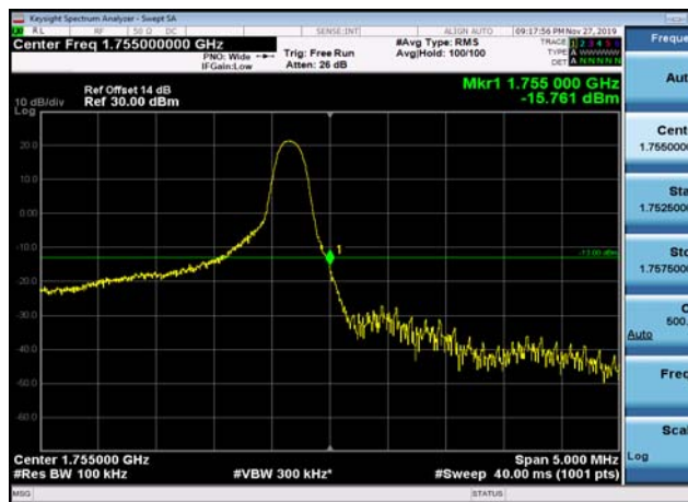
HighRange_FDD04_5MHz_1752.5_OneRB_high_QPSK
