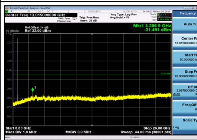
FDD05_MidRange_1.4MHz_30MHz~26GHz
