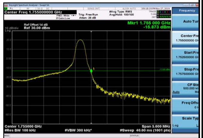
HighRange_FDD04_5MHz_1752.5_OneRB_high_Q16
