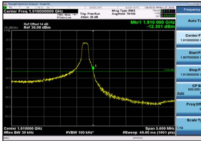
HighRange_FDD02_3MHz_1908.5_fullIRB_High_QPSK
