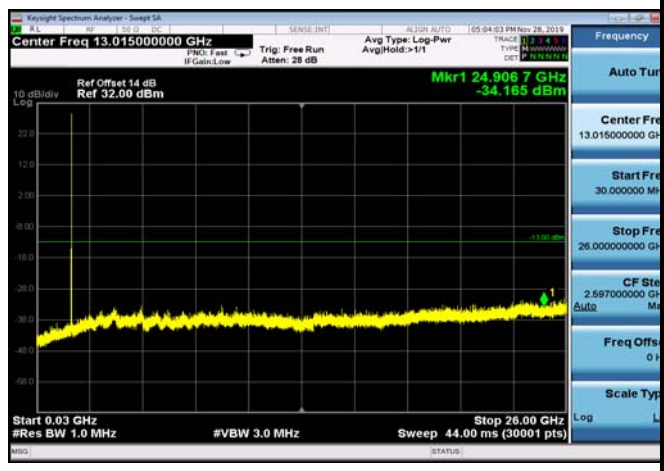
FDD04_MidRange_5MHz_30MHz~26GHz
