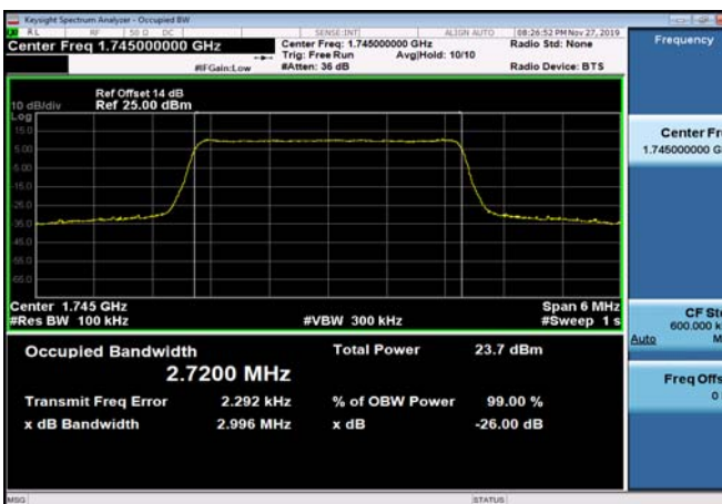
FDD66_MidRange_3MHz_1745MHz_QPSK
