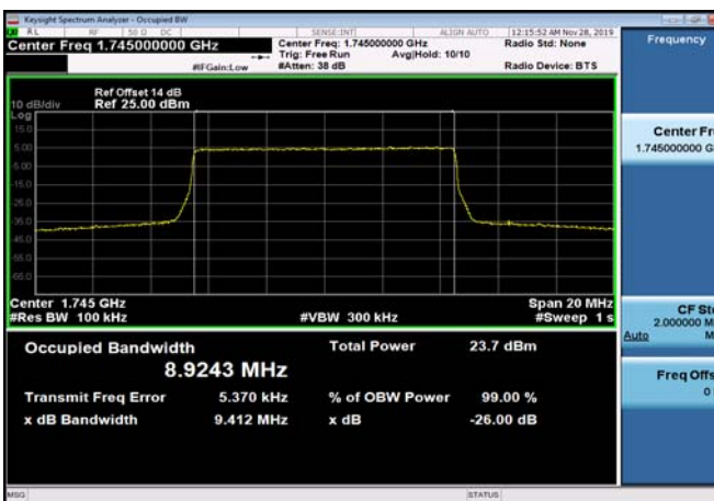
FDD66_MidRange_10_1745_QPSK
