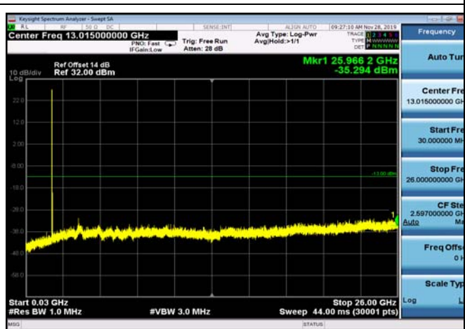
FDD02_LowRange_5MHz_30MHz~26GHz
