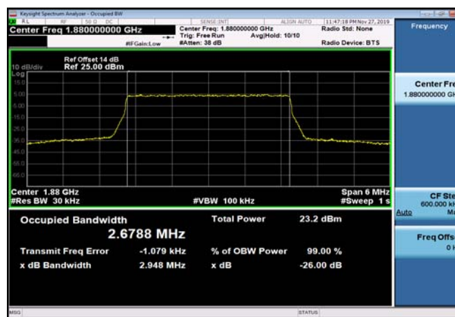
FDD02_MidRange_5_1880_Q16
