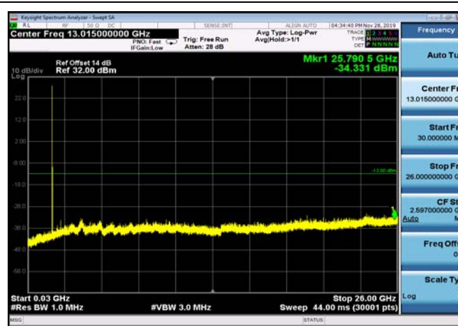
FDD04_HighRange_15MHz_30MHz~26GHz
