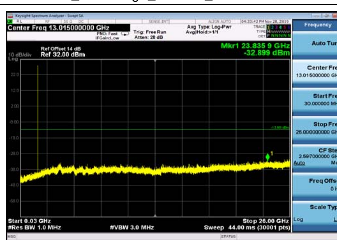
FDD04_LowRange_15MHz_30MHz~26GHz
