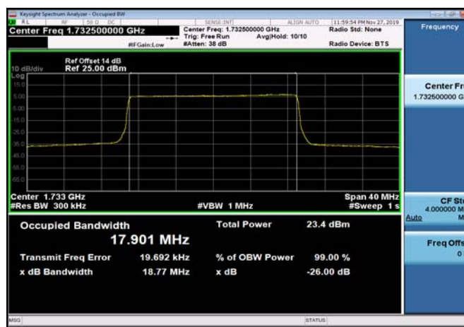
FDD04_MidRange_20_1732.5_QPSK
