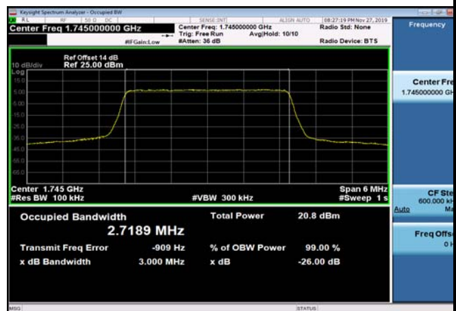
FDD66_MidRange_3MHz_1745MHz_Q16
