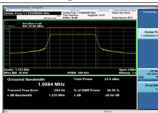
FDD04_MidRange_1.4MHz_1732.5MHz_QPSK
