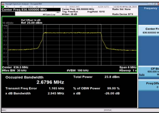
FDD05_MidRange_5_836.5_QPSK
