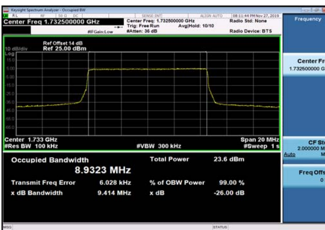
FDD04_MidRange_10MHz_1732.5MHz_QPSK
