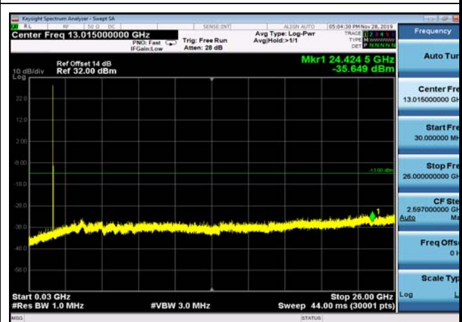
FDD04_HighRange_5MHz_30MHz~26GHz
