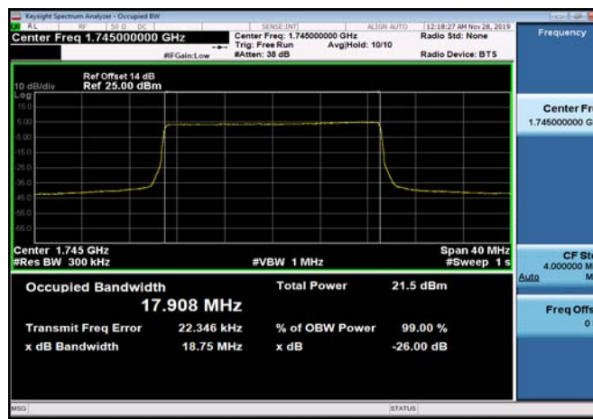
FDD66_MidRange_20_1745_QPSK
