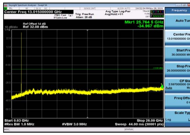
FDD04_MidRange_3MHz_30MHz~26GHz
