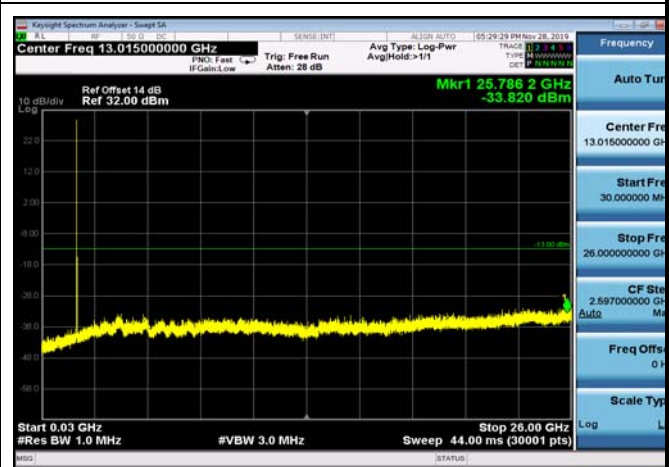
FDD04_HighRange_20MHz_30MHz~26GHz
