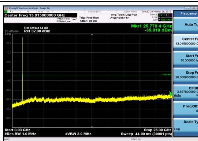
FDD04_HighRange_3MHz_30MHz~26GHz
