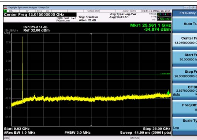
FDD02_MidRange_3MHz_30MHz~26GHz
