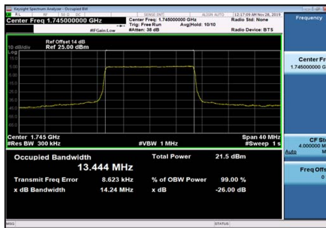
FDD66_MidRange_20_1745_QPSK
