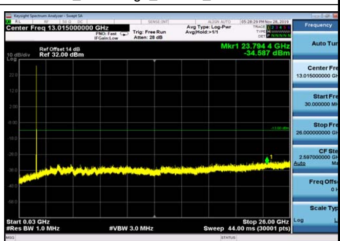
FDD04_LowRange_20MHz_30MHz~26GHz
