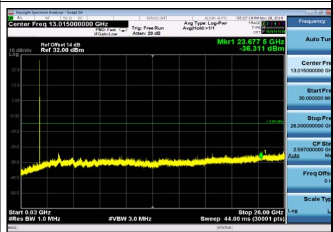
FDD02_MidRange_20MHz_30MHz~26GHz
