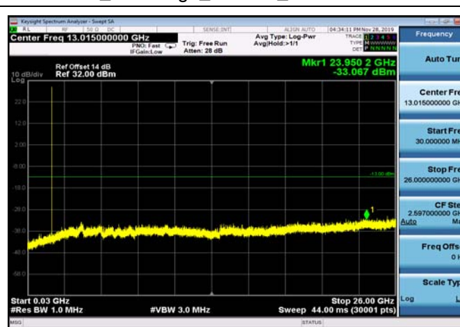
FDD04_MidRange_15MHz_30MHz~26GHz
