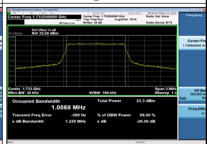
FDD04_MidRange_1.4MHz_1732.5MHz_Q16
