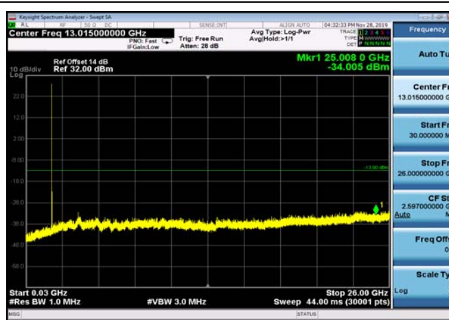
FDD02_MidRange_15MHz_30MHz~26GHz
