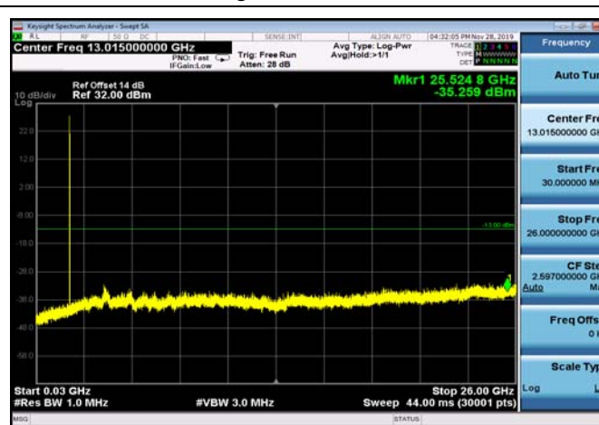
FDD02_LowRange_15MHz_30MHz~26GHz
