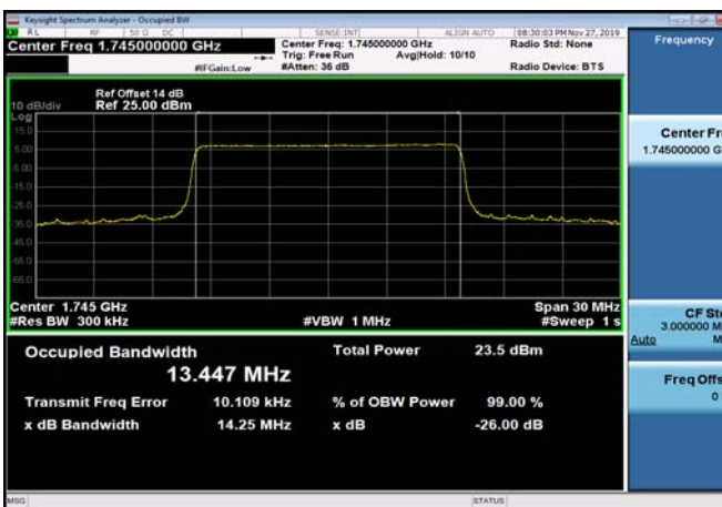
FDD66_MidRange_15MHz_1745MHz_QPSK
