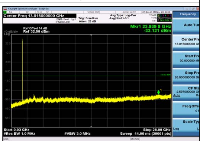
FDD02_LowRange_20MHz_30MHz~26GHz
