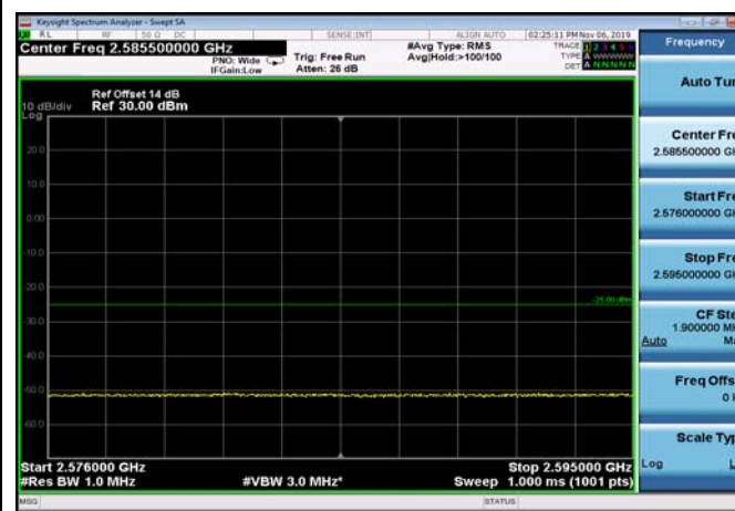
LowRange_FDD07_15MHz_2507.5_OneRB _low_Q16
