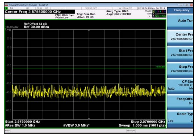
FDD07_20MHz_2560_Q16_OneRB_high _ExtraBands_Range_2575~2576
