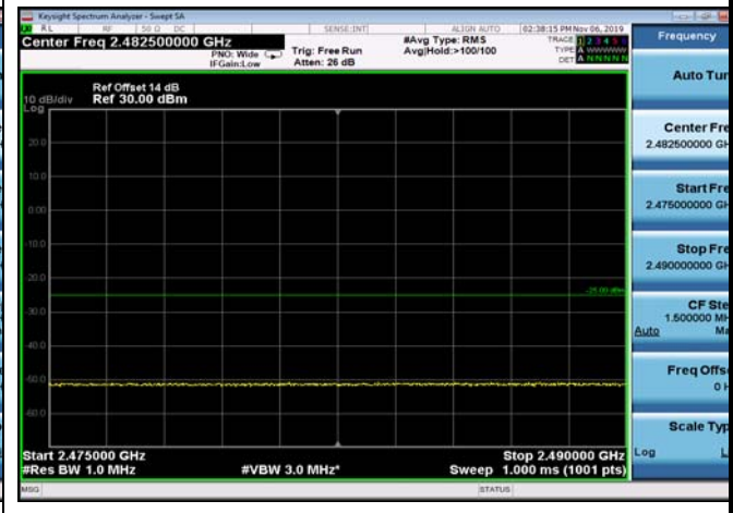
FDD07_5MHz_2567.5_QPSK_fullRB_ExtraBa nds_Range_2475~2490
