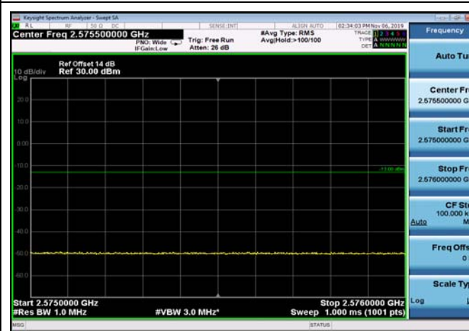
HighRange_FDD07_5MHz_2567.5_OneRB _high_QPSK
