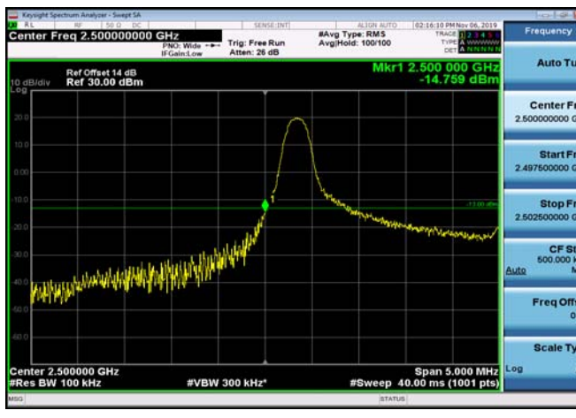
LowRange_FDD07_5MHz_2502.5_OneRB _low_Q16
