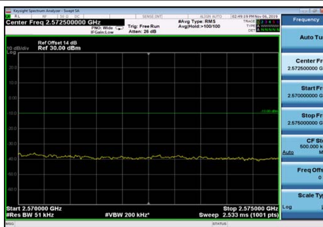
FDD07_15MHz_2562.5_QPSK_fullIRB _ExtraBands_Range_2570~2575
