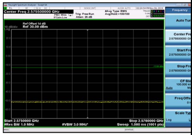
FDD07_15MHz_2507.5_QPSK_OneRB_high _ExtraBands_Range_2575~2576
