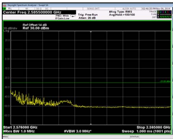
FDD07_15MHz_2562.5_Q16_OneRB_high_ExtraBands_Range_2576~2595
