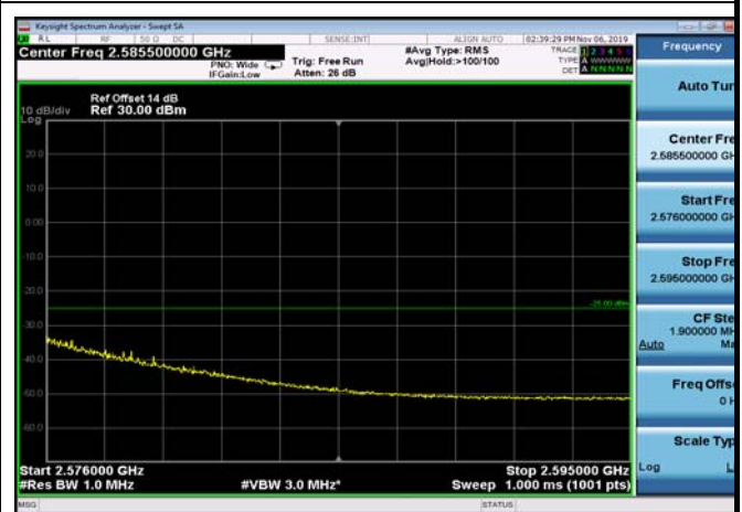
HighRange_FDD07_10MHz_2565_OneRB_high_Q16
