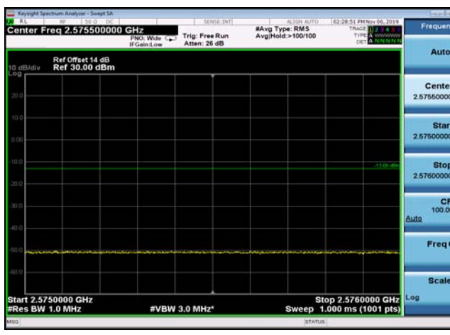
FDD07_15MHz_2507.5_Q16_fullRB_ExtraBands_Range_2575~2576
