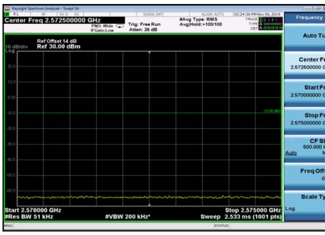
FDD07_15MHz_2507.5_QPSK_OneRB_high _ExtraBands_Range_2570~2575
