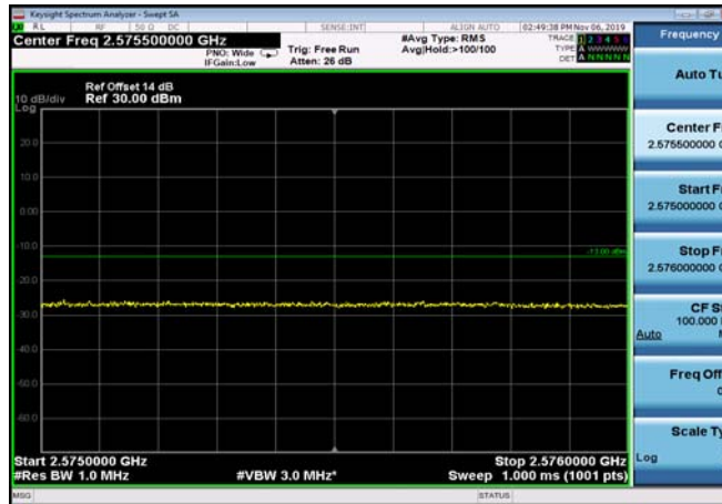
HighRange_FDD07_20MHz_2560_OneRB _high_QPSK
