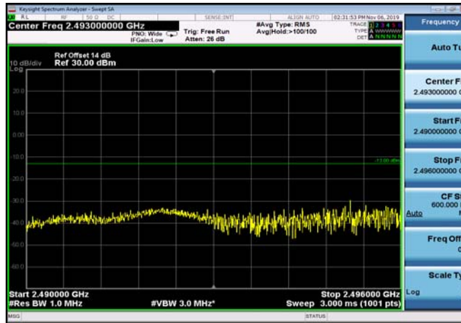
LowRange_FDD07_20MHz_2510_fullRB _Low_Q16
