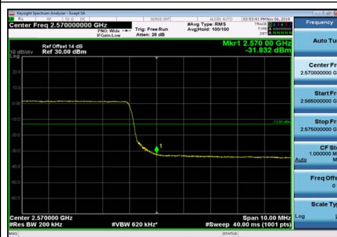
HighRange_FDD07_20MHz_2560_fullIRB _High_Q16
