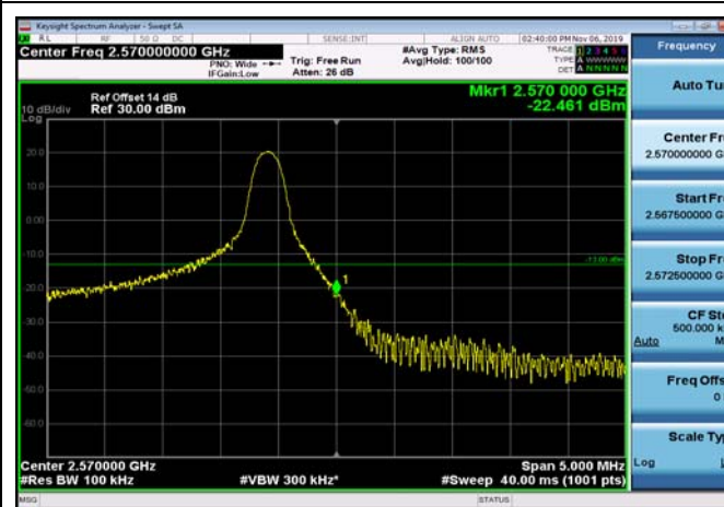
HighRange_FDD07_10MHz_2565_OneRB_high_QPSK
