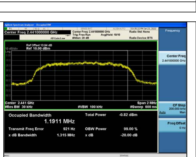
Test Mode:8DPSK(3DH5) MHz
