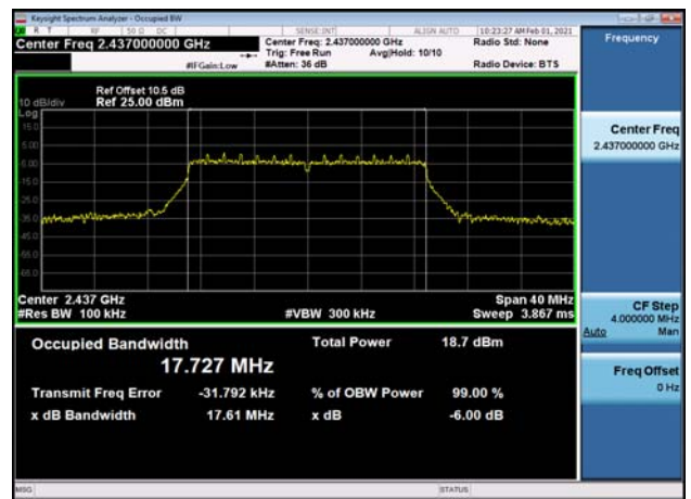
6dB Bandwidth-802.11n(HT20),2437MHz
