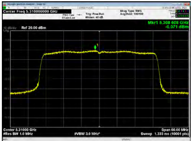
U-NII-2A, 802.11ax HE40, Channel No.: 62
