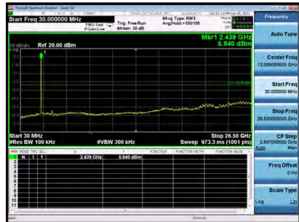
802.11ax(HE20)-242Tone, Channel No. 9
