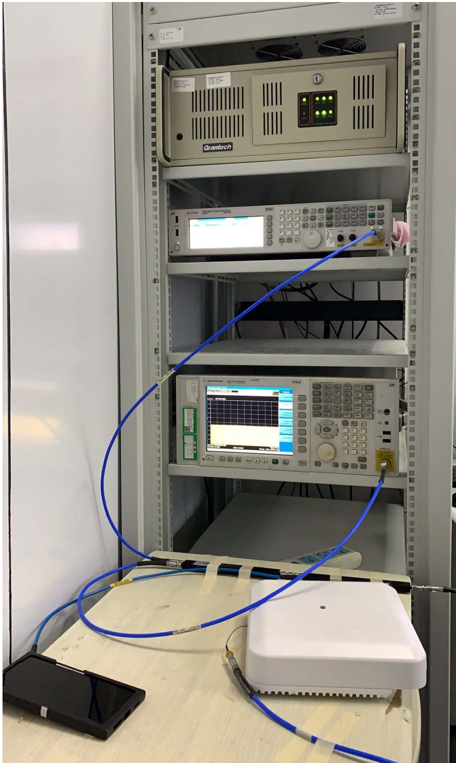
Picture 1 Test Setup
