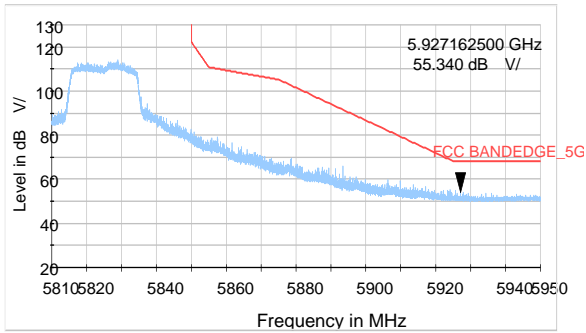
802.11ax HE40-Channel 159: Peak
