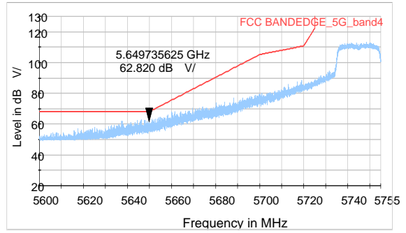
802.11ax HE40-Channel 151: Peak
