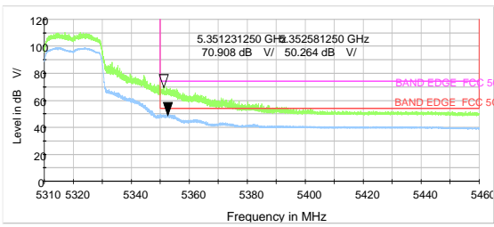
802.11ax HE40-Channel 62: Peak/Average
