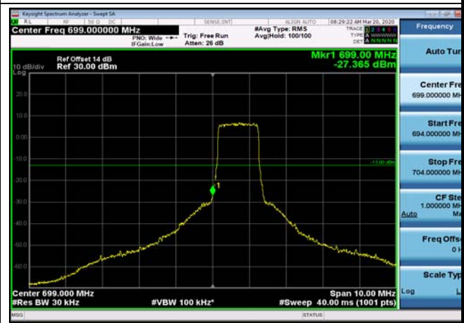
LowRange_FDD12_1.4MHz_699.7_fullIRB _Low_Q16
