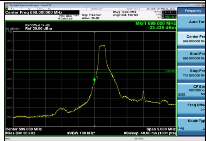
LowRange_FDD12_3MHz_700.5_fullRB _Low_Q16
