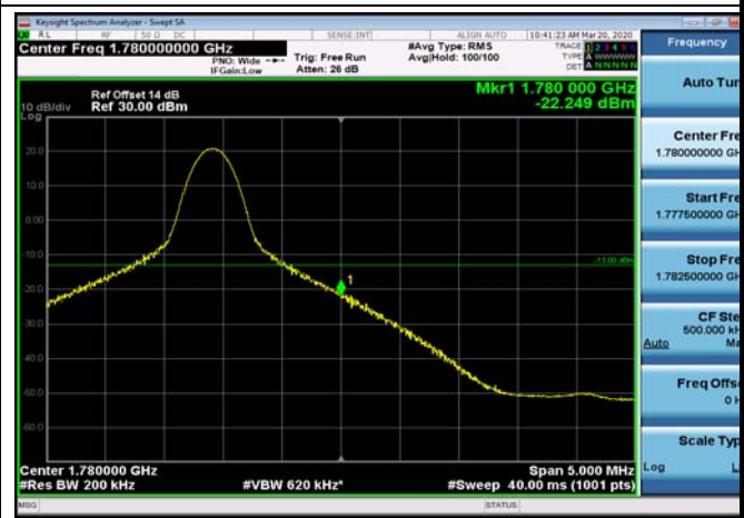
HighRange_FDD66_20MHz_1770_OneRB _high_Q16
