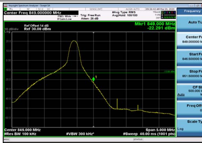
HighRange_FDD26_10MHz_844_OneRB _high_QPSK
