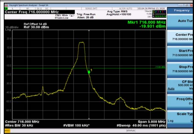
HighRange_FDD12_3MHz_714.5_OneRB _high_Q16
