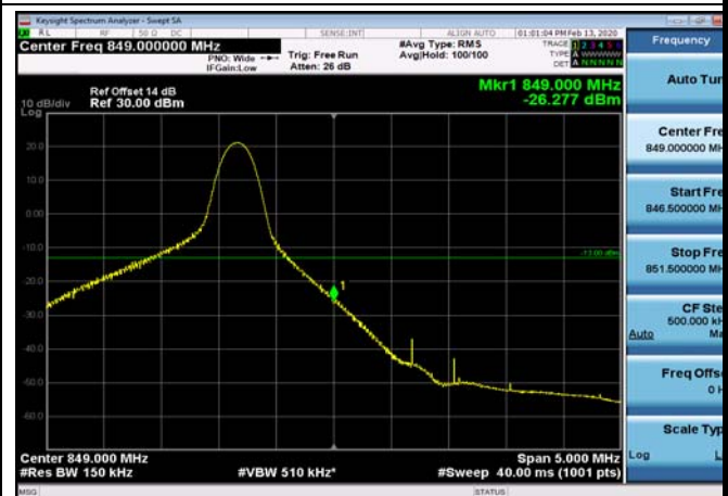
HighRange_FDD26_15MHz_841.5_fullIRB _High_Q16
