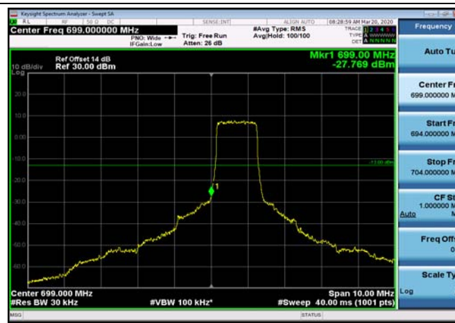
LowRange_FDD12_1.4MHz_699.7_fullIRB _Low_QPSK
