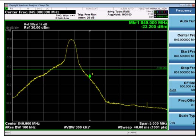
HighRange_FDD26_10MHz_844_OneRB _high_Q16
