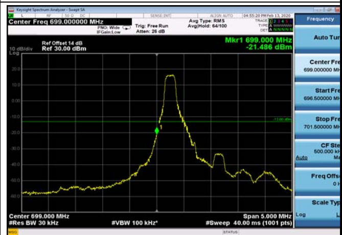
LowRange_FDD12_1.4MHz_699.7_fullIRB _Low_Q16
