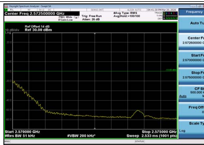
FDD07_10MHz_2565_Q16_OneRB_high_ExtraBands_Range_2570~2575
