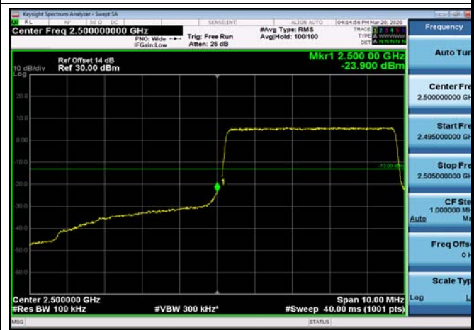
LowRange_FDD07_5MHz_2502.5_fullIRB _Low_QPSK
