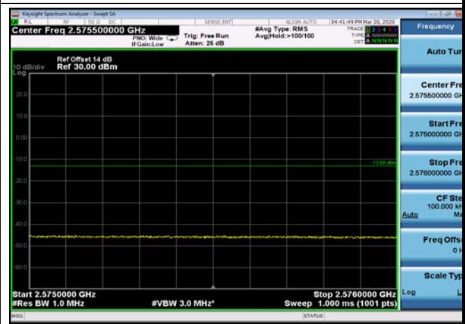
FDD07_10MHz_2565_Q16_OneRB_high_ExtraBands_Range_2575~2576
