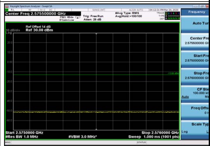
FDD07_5MHz_2502.5_QPSK_OneRB_high _ExtraBands_Range_2575~2576
