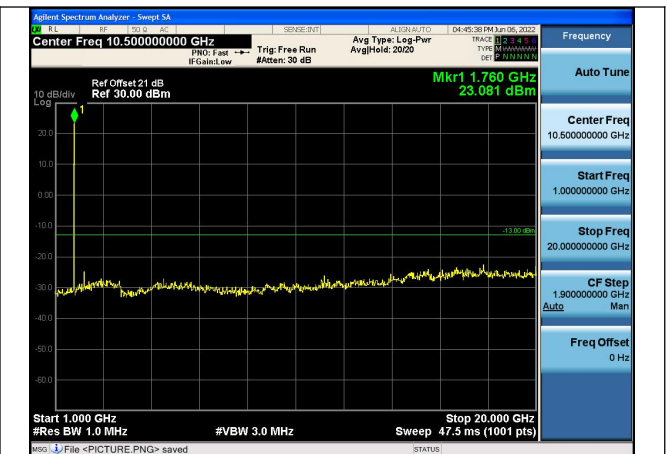
Channel 1312 1GHz~20GHz(dBm)
