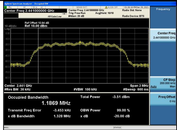
Test Mode:π/4DQPSK(2DH5) MHz
