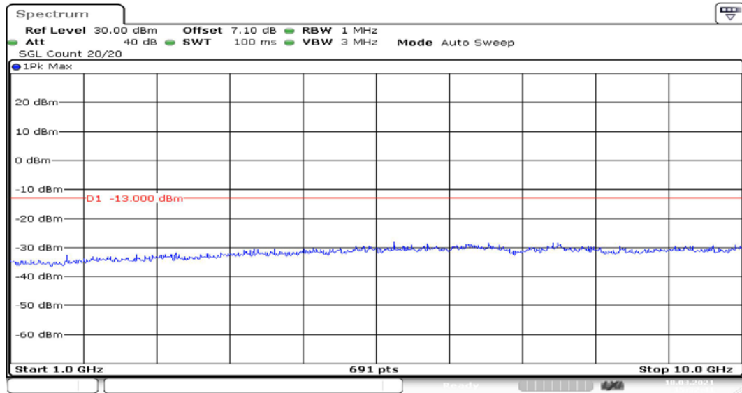
Channel 189 1GHz~10GHz
