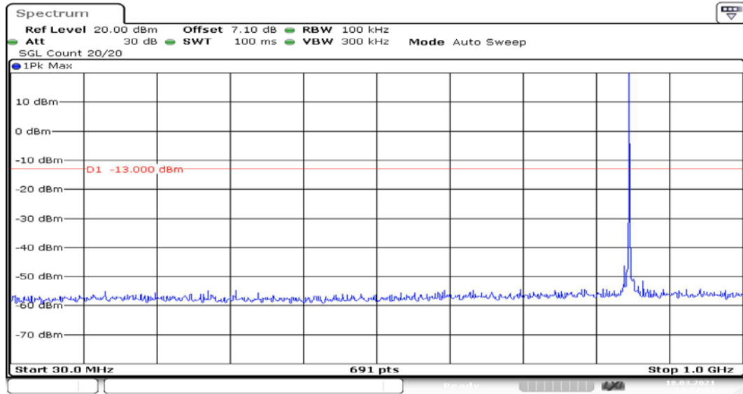
Channel 189 30MHz~1GHz
