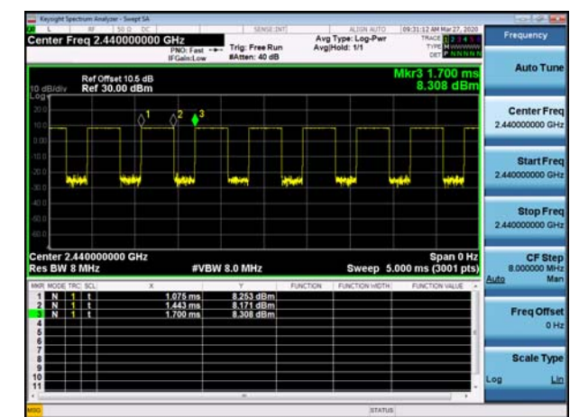
Dutycycle=58.9%
