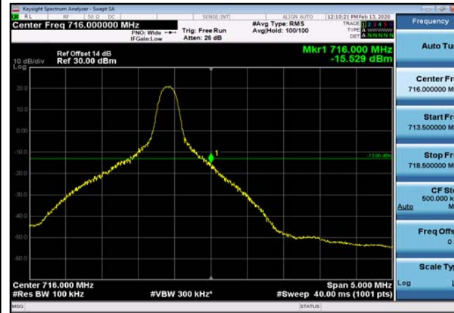
HighRange_FDD12_10MHz_711_fullRB _High_QPSK
