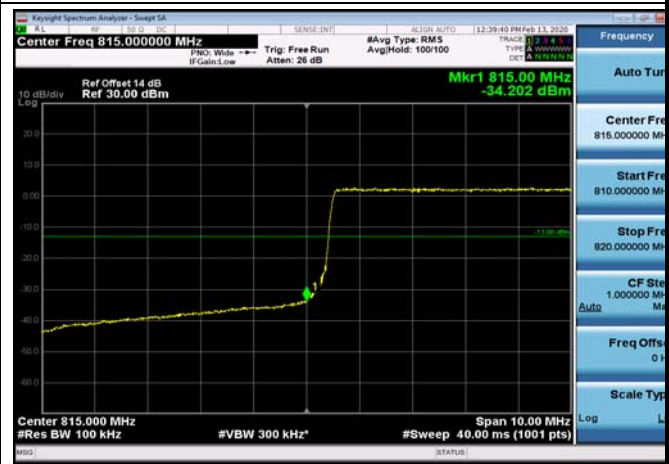
LowRange_FDD26_10MHz_820_fullRB _Low_Q16
