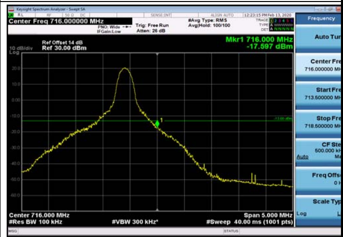
HighRange_FDD17_10MHz_711_OneRB _high_Q16
