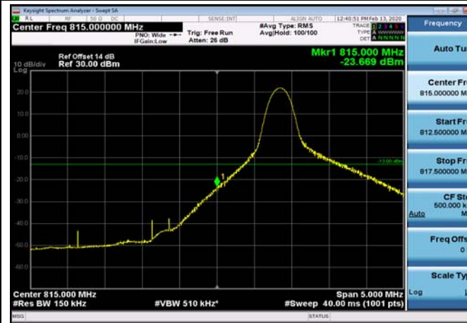
LowRange_FDD26_15MHz_822.5_fullIRB _Low_QPSK
