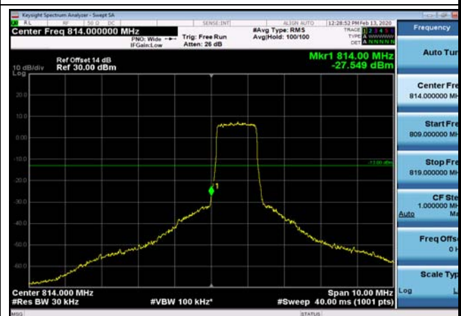
LowRange_FDD26_1.4MHz_814.7_fullRB _Low_Q16
