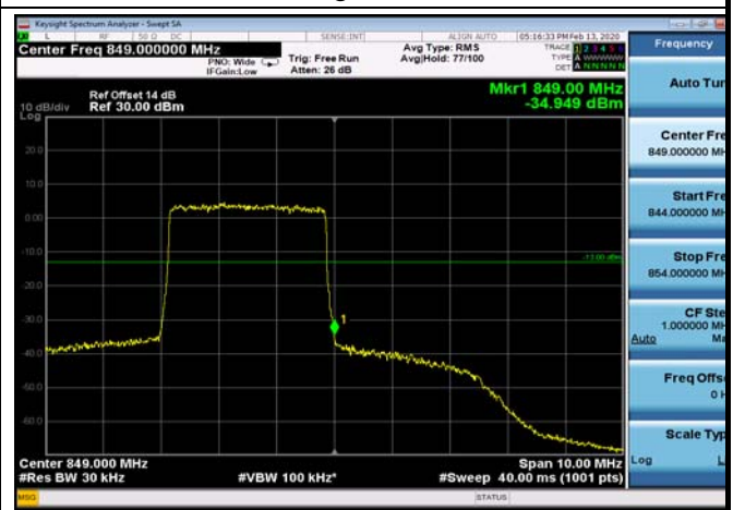
HighRange_FDD26_3MHz_847.5_fullRB _High_Q16
