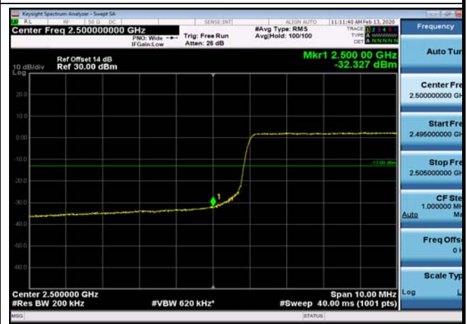
LowRange_FDD07_20MHz_2510_fullRB _Low_QPSK
