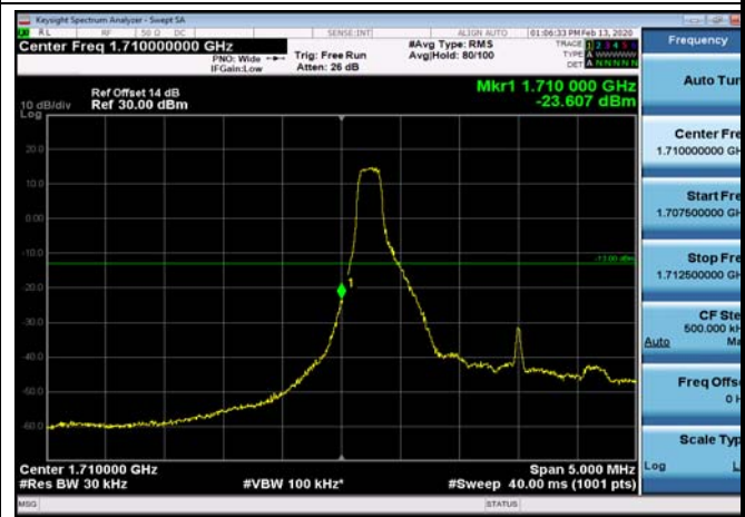
LowRange_FDD66_3MHz_1711.5_OneRB _low_Q16
