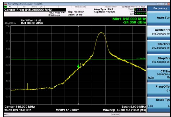
LowRange_FDD26_15MHz_822.5_fullIRB _Low_Q16
