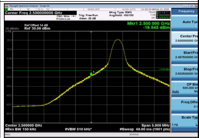
LowRange_FDD07_15MHz_2507.5_OneRB _low_QPSK
