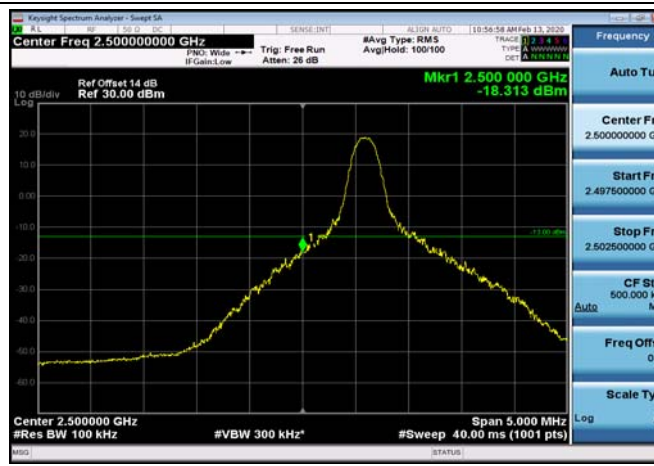
LowRange_FDD07_10MHz_2505_OneRB _low_Q16
