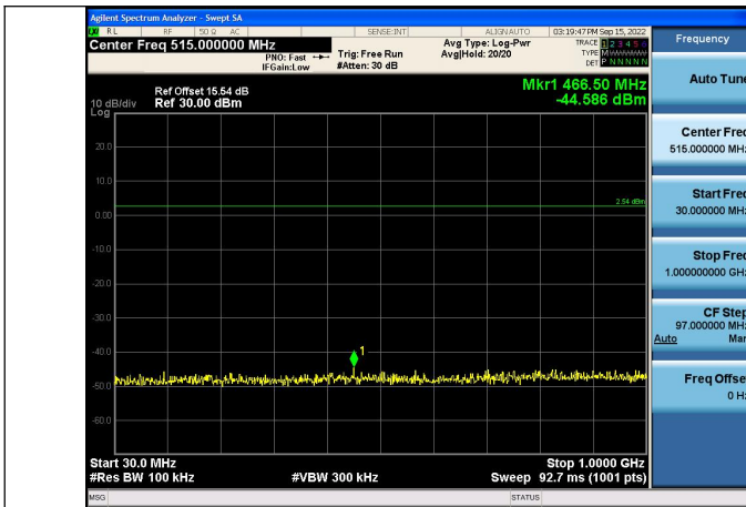
Channel 9262 30MHz~1GHz
