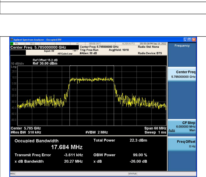
Test Mode:802.11n HT20 5785MHz Chain0
