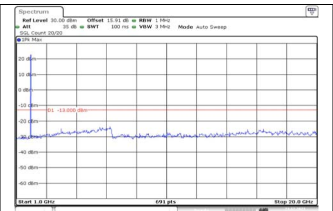
Channel 9262 1GHz~20GHz(dBm)
