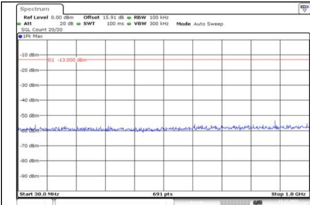
Channel 9262 30MHz~1GHz(dBm)
