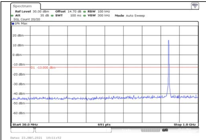
Channel 4132 30MHz~1GHz(dBm)
