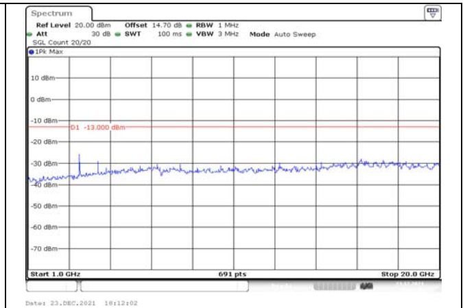
Channel 4132 1GHz~20GHz(dBm)
