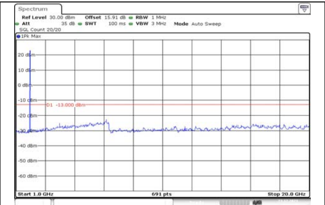
Channel 9262 1GHz~20GHz(dBm)
