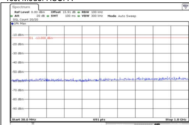
Channel 9262 30MHz~1GHz(dBm)
