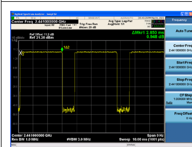
Modulation: 8DPSK DH5 2441
