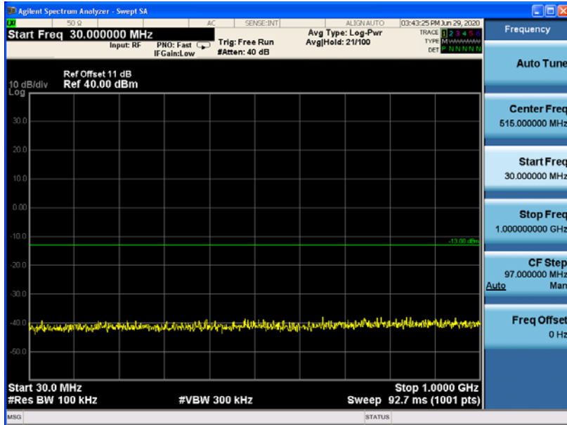
Channel 1412, 30MHz~1GHz
