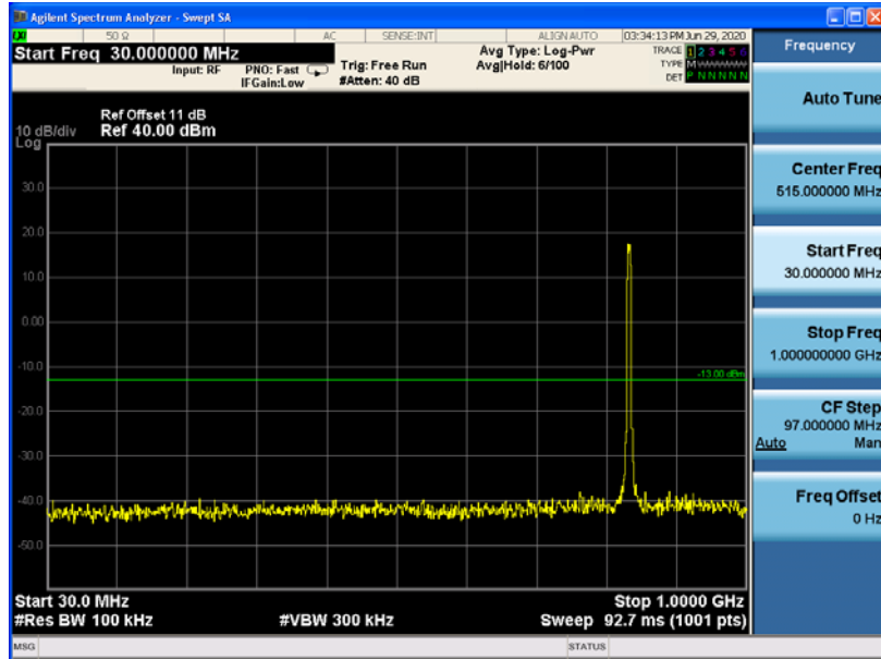
Channel 4183, 30MHz~1GHz
