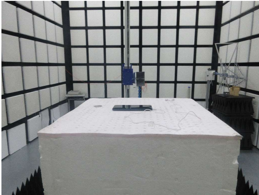
Field Strength of Spurious Radiation (Above 1GHz)
