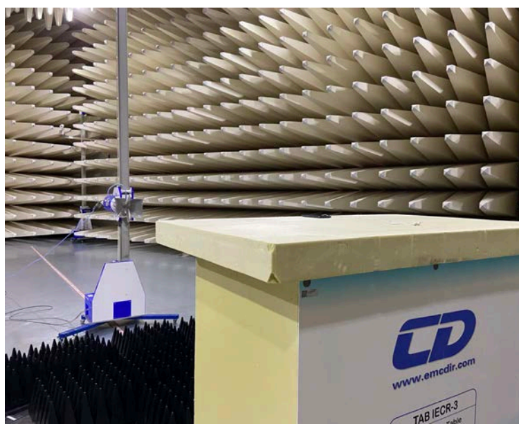
Radiated Emissions Test Setup ( above1GHz)
