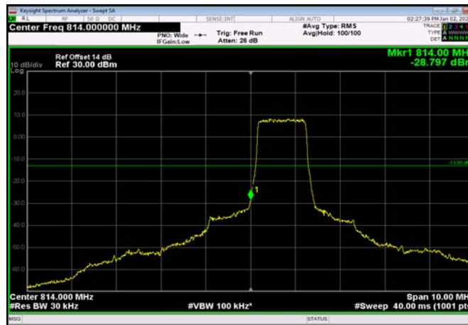
LowRange_FDD26_3MHz_815.5_OneRB _low_QPSK
