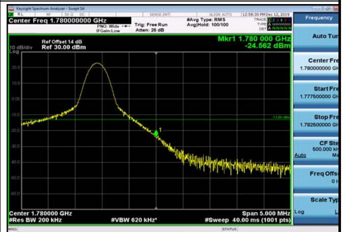
HighRange_FDD66_20MHz_1770_fullIRB _High_Q16
