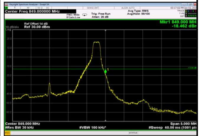
HighRange_FDD26_3MHz_847.5_fullIRB _High_Q16
