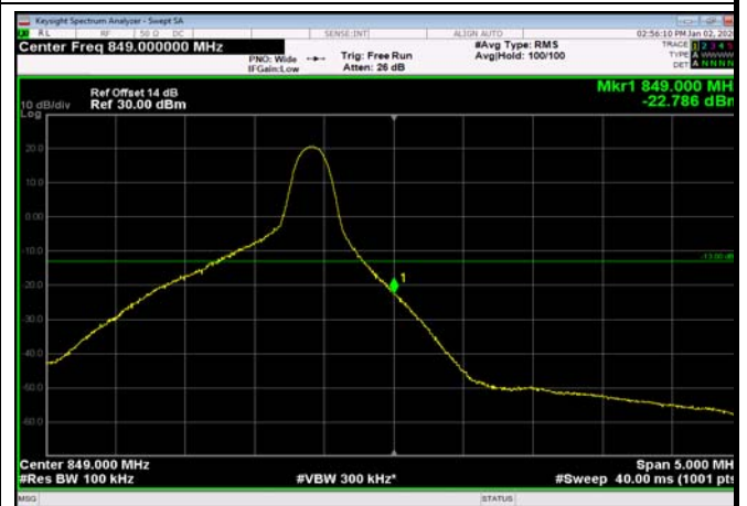
HighRange_FDD26_10MHz_844_fullRB _High_Q16
