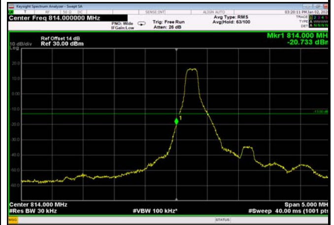
LowRange_FDD26_1.4MHz_814.7_fullIRB _Low_Q16
