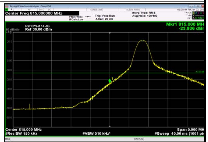
LowRange_FDD26_15MHz_822.5_OneRB _low_Q16
