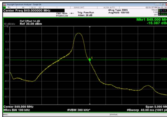
HighRange_FDD26_5MHz_846.5_OneRB _high_QPSK
