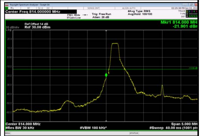
LowRange_FDD26_3MHz_815.5_OneRB _low_Q16
