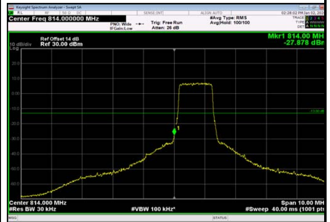
LowRange_FDD26_3MHz_815.5_OneRB _low_Q16
