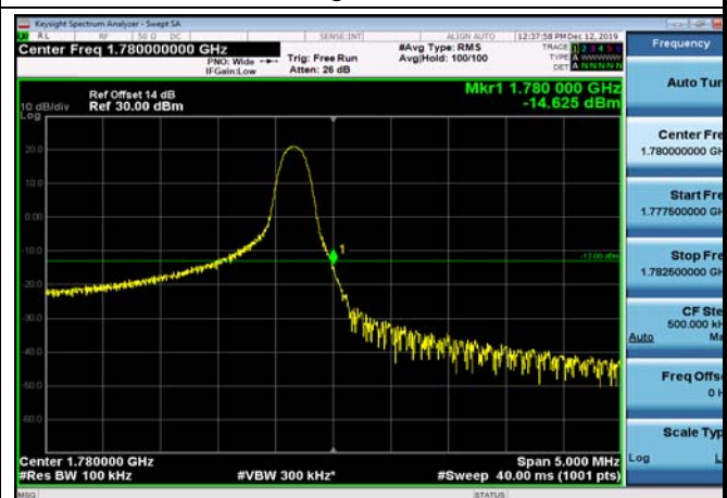
HighRange_FDD66_5MHz_1777.5_OneRB _high_Q16
