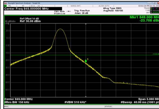
HighRange_FDD26_15MHz_841.5_fullIRB _High_QPSK
