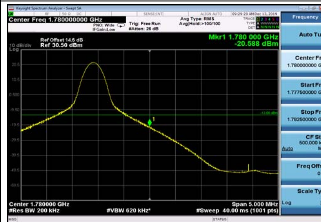
HighRange_FDD66_20MHz_1770_fullIRB _High_QPSK
