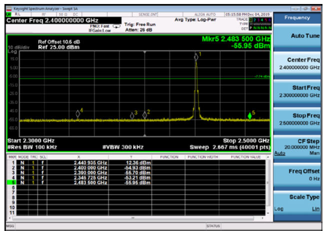
Conducted Emission: DQPSK,2441,2DH5 ,Band Edge HoppingOFF
