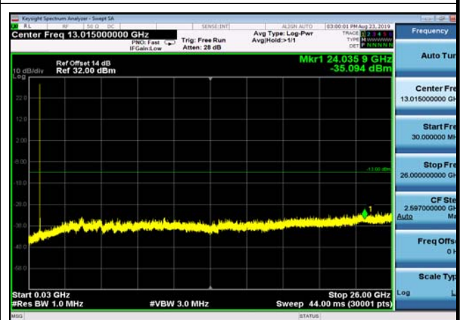
FDD05_LowRange_10MHz_30MHz~26GHz
