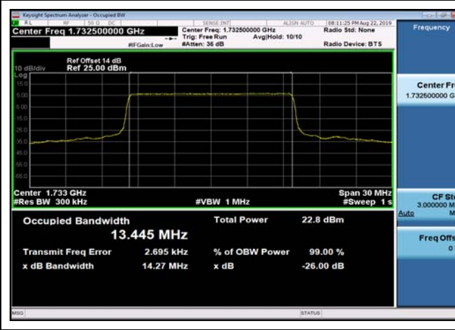
FDD04_MidRange_15MHz_1732.5MHz_QPSK
