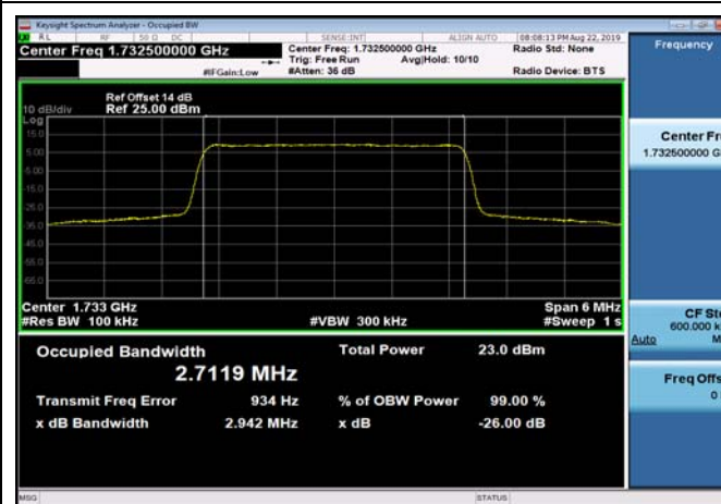
FDD04_MidRange_3MHz_1732.5MHz_QPSK
