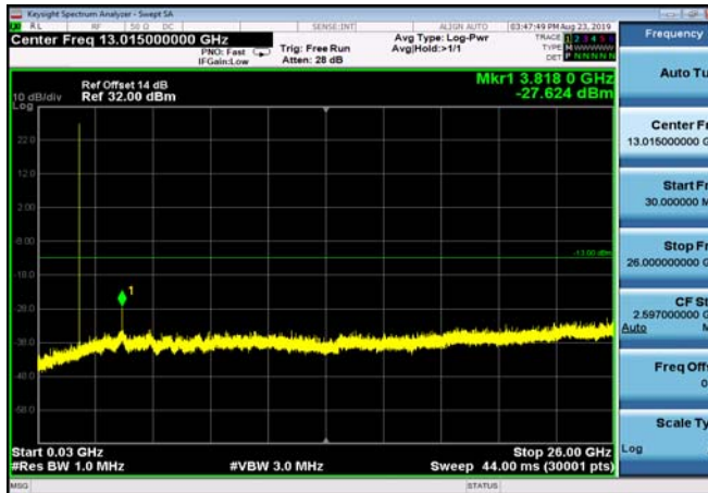
FDD02_HighRange_15MHz_30MHz~26GHz
