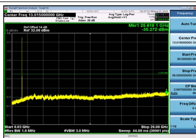
FDD04_LowRange_3MHz_30MHz~26GHz
