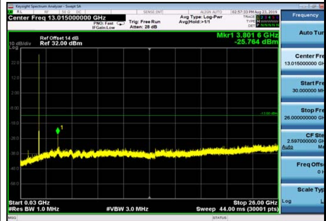
FDD02_HighRange_20MHz_30MHz~26GHz
