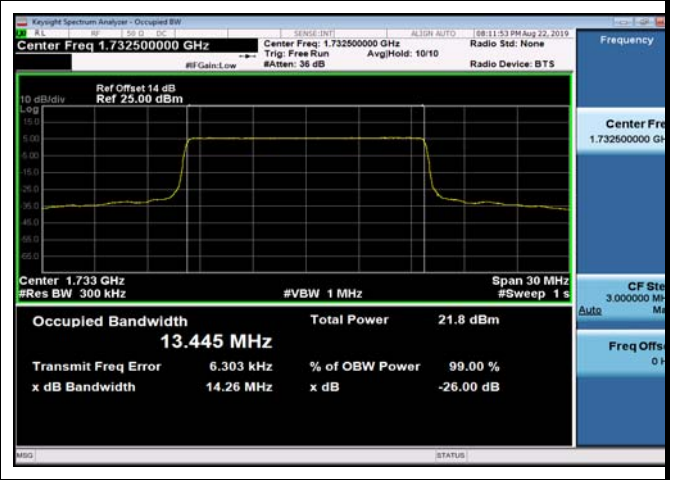
FDD04_MidRange_15MHz_1732.5MHz_Q16
