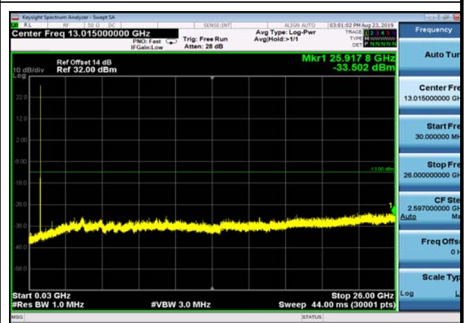
FDD05_HighRange_5MHz_30MHz~26GHz
