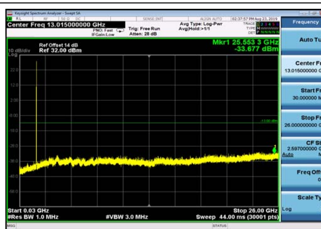
FDD04_MidRange_3MHz_30MHz~26GHz
