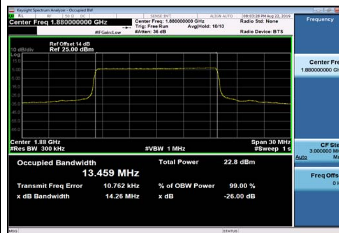
FDD02_MidRange_15MHz_1880MHz_QPSK
