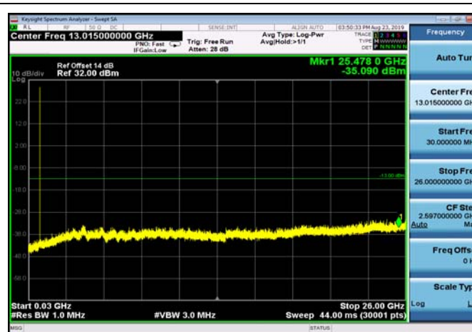
FDD05_LowRange_1.4MHz_30MHz~26GHz
