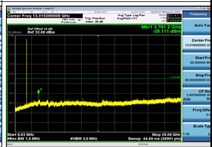
FDD02_LowRange_20MHz_30MHz~26GHz
