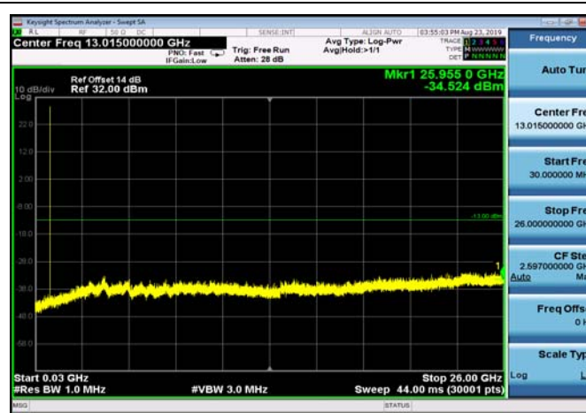
FDD05_HighRange_3MHz_30MHz~26GHz
