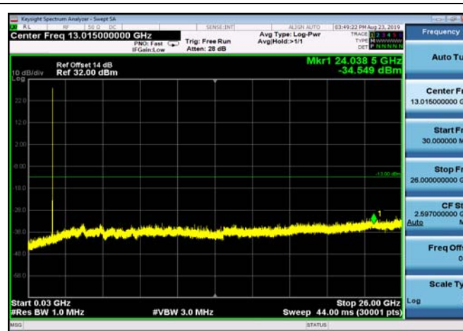
FDD04_MidRange_15MHz_30MHz~26GHz
