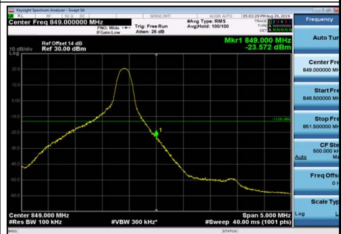
HighRange_FDD26_10MHz_844_OneRB _high_Q16
