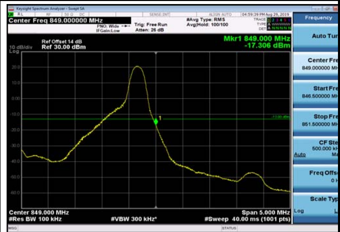
HighRange_FDD26_5MHz_846.5_fullIRB _High_Q16
