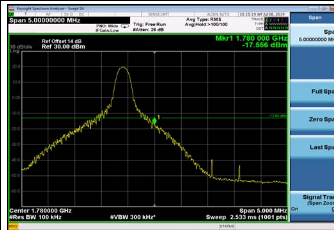
HighRange_FDD66_10MHz_1775_fullIRB _High_QPSK
