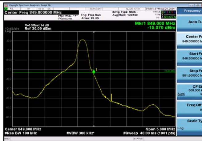
HighRange_FDD26_5MHz_846.5_fullIRB _High_QPSK
