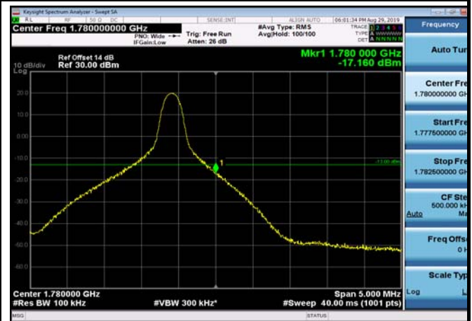
HighRange_FDD66_10MHz_1775_fullIRB _High_Q16
