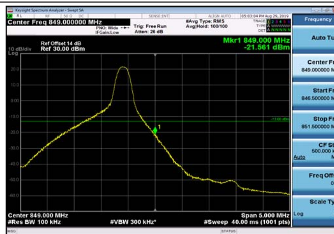
HighRange_FDD26_10MHz_844_OneRB _high_QPSK
