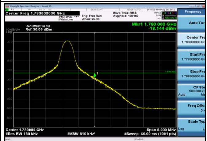
HighRange_FDD66_15MHz_1772.5_OneRB _high_Q16
