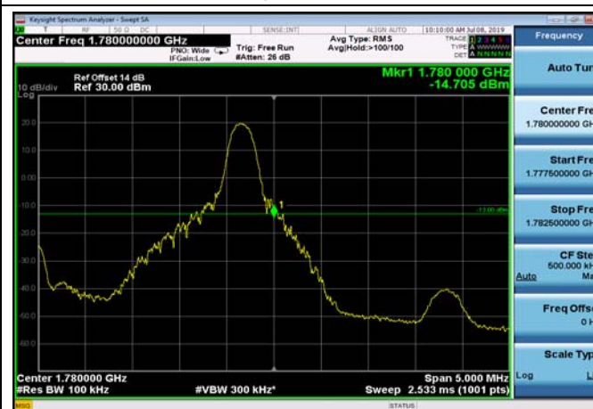
HighRange_FDD66_5MHz_1777.5_fullRB_High_QPSK
