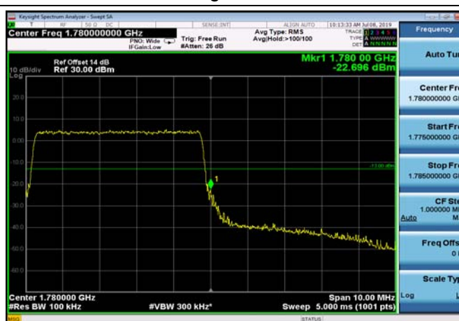
HighRange_FDD66_5MHz_1777.5_fullRB_High_Q16
