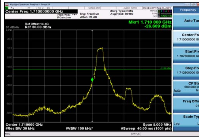
LowRange_FDD66_1.4MHz_1710.7_fullRB _Low_QPSK
